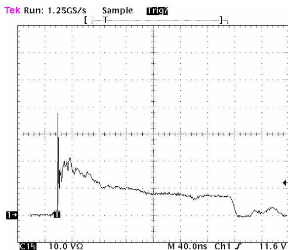
Figure 2. Positive 8 kV contact per IEC 6100-4-2 - ESD5Z5VA-2/TR
