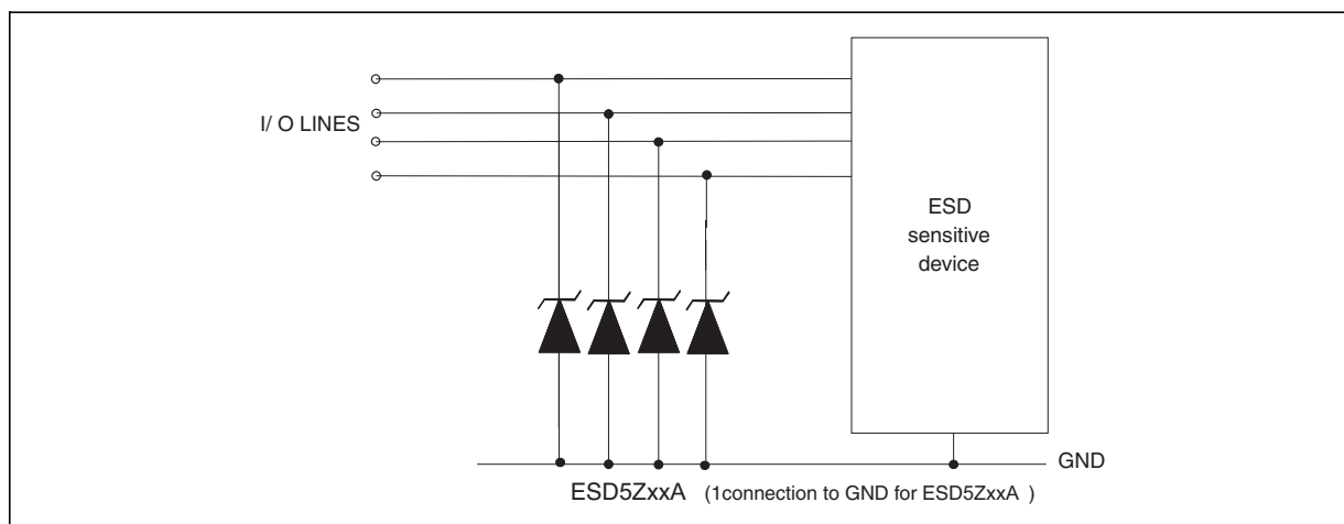
Figure4: ESD5ZxxA protection against ESD
