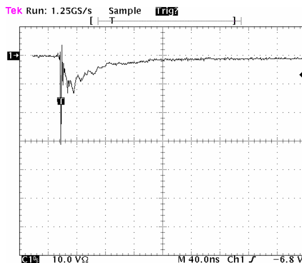
Figure 3. Negative 8 kV contact per IEC 6100-4-2 - ESD5Z5VA-2/TR
