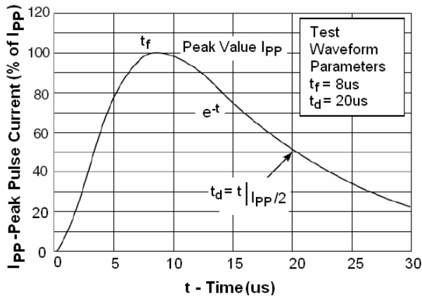
Figure1. Pulse Waveform
