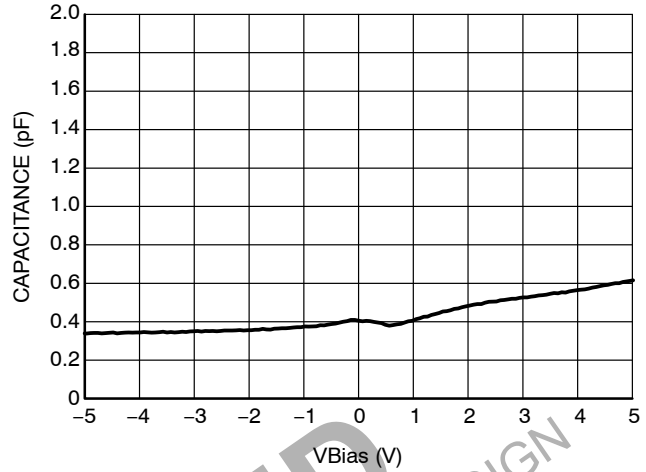
Figure 4. CV Characteristics
