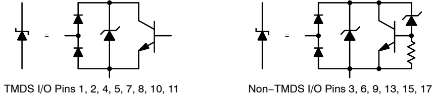
Figure 1. Pin Schematic
