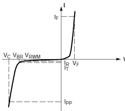
Uni-Directional TVS
