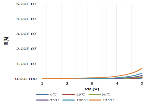
Figure4. Leakage Current
