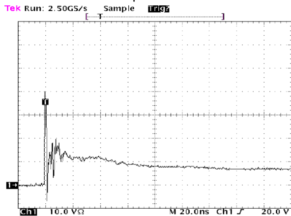
Figure3. Forward Characteristics
