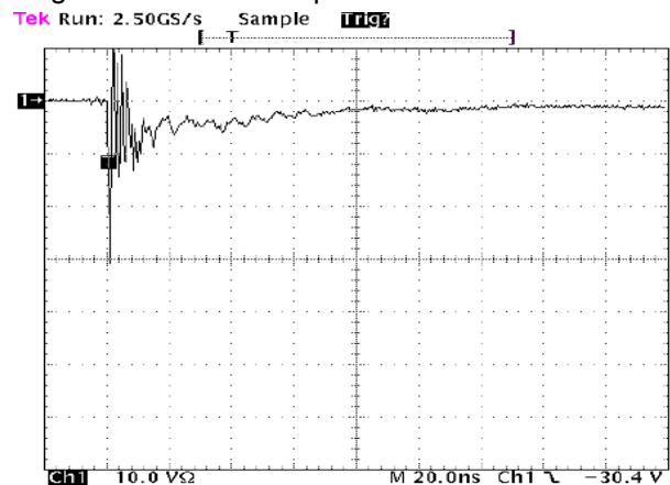
Figure4. Leakage Current
