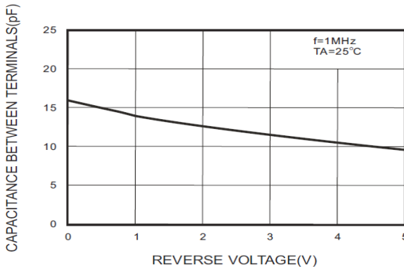
FIG.3- TERMINALS CHARACTERISTICS
