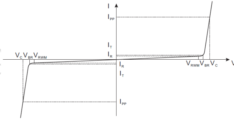
Bi-Directional TVS
