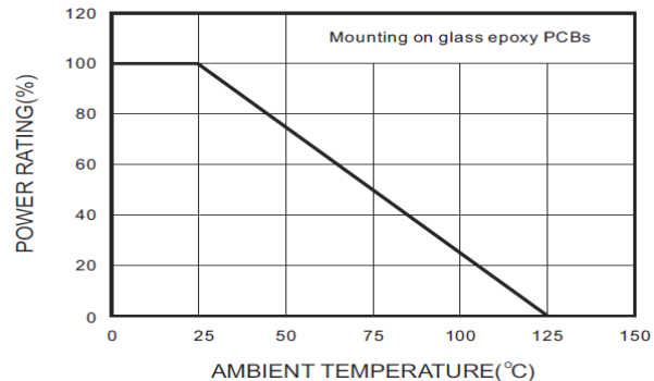
FIG.4- POWER RATING DERATING CURVE
