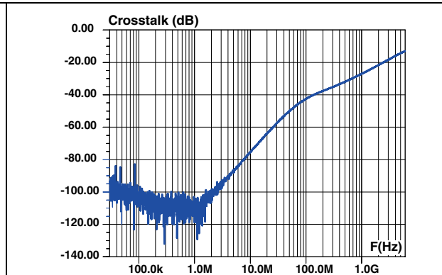
Figure 10. Analog crosstalk measurements between channels
