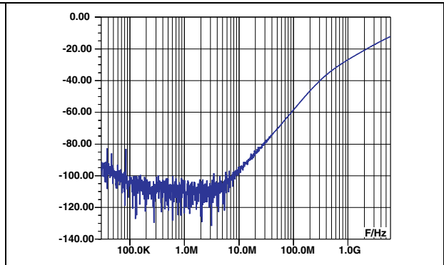
Figure 10. Analog crosstalk measurements between channels
