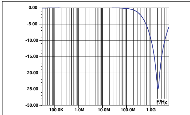
Figure 9. S21 attenuation measurement results of each channel
