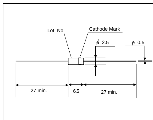
Outline Drawings : mm
