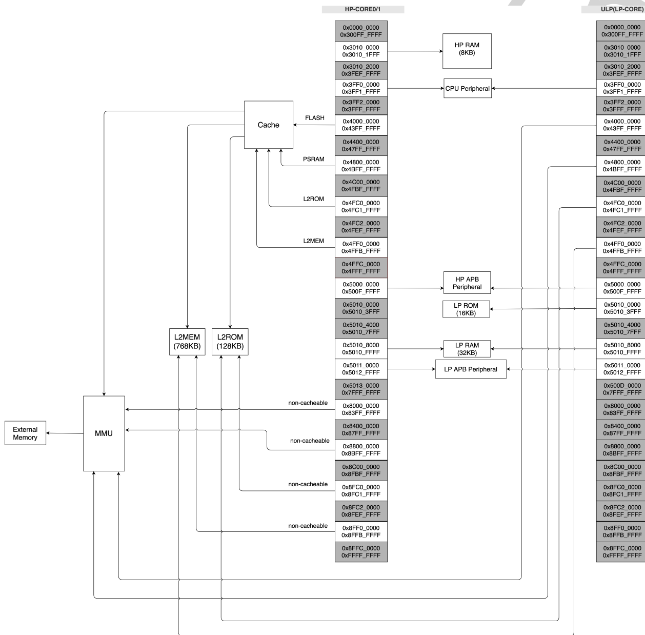
Figure 3-1. Address Mapping Structure
