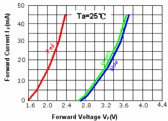
< Figure 7 Forward voltage & forward current for PLCC 5050 series >
