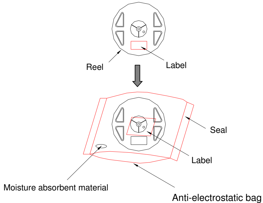
< Figure 11 Packaging diagram >
