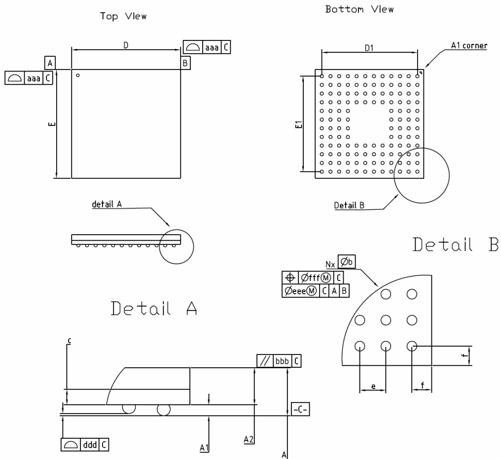
Figure 54: Package Outline
