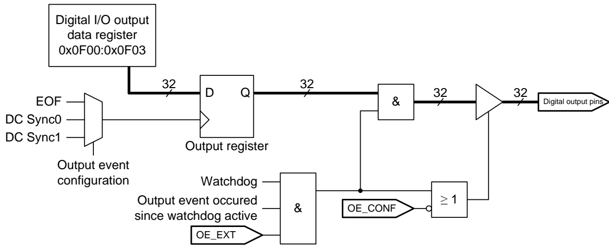
Figure 10: Digital Output Principle Schematic
