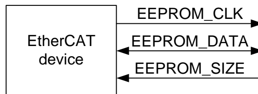
Figure 42: I 2 C EEPROM signals
