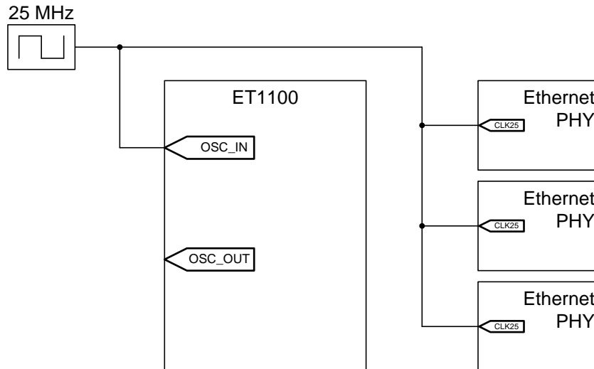
Figure 45: Oscillator clock source for ET1100 and Ethernet PHYs
