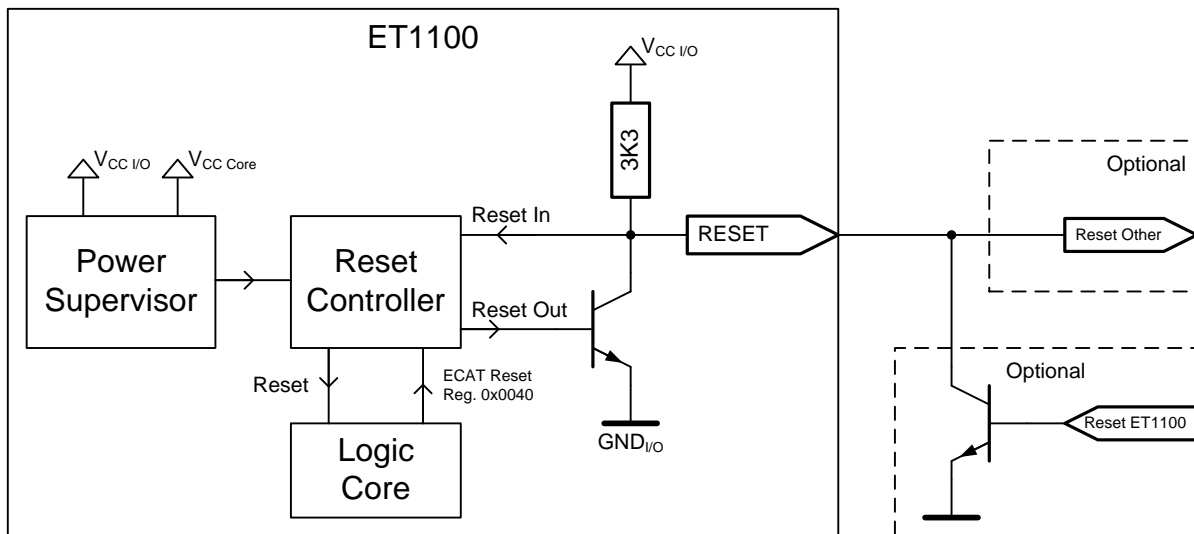
Figure 51: Reset Logic
