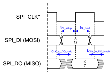
Figure 17: Basic SPI_DI/SPI_DO timing (*refer to timing diagram for relevant edges of SPI_CLK)
