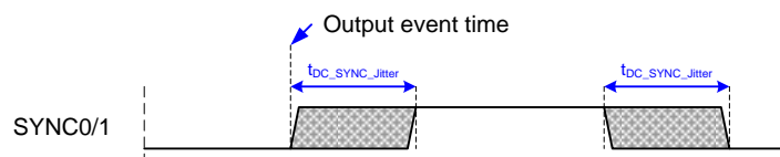
Figure 41: SyncSignal timing
