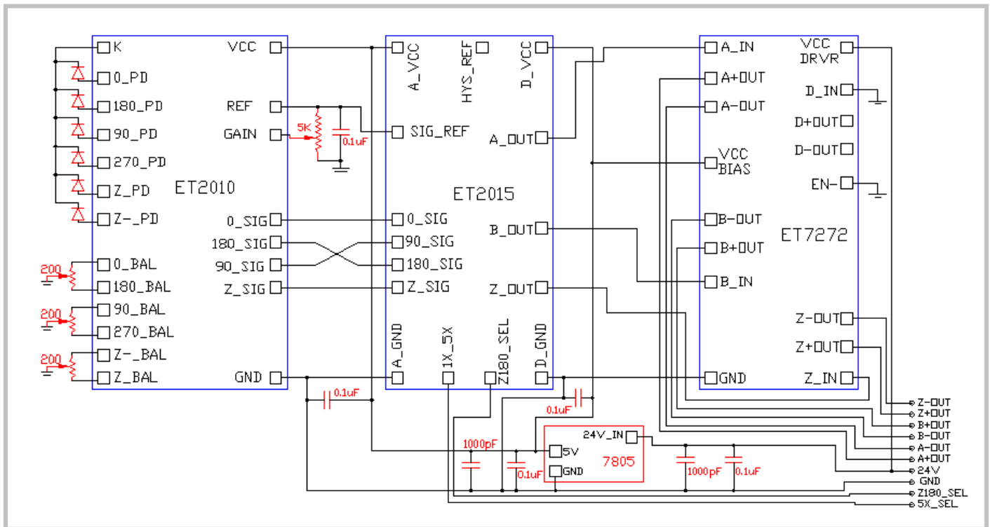
Application Circuit
