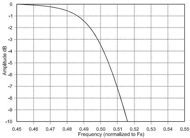
Transition Band
