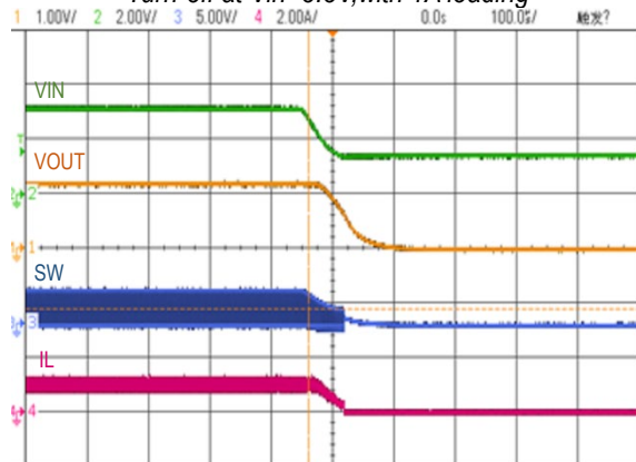
Turn-off at Vin=3.3V, with 1A loading
