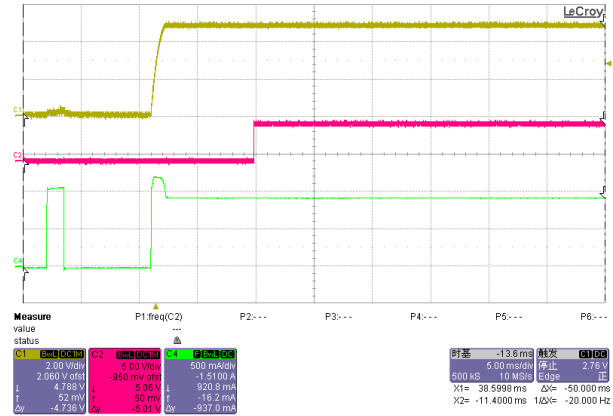
Short-Circuit to Full load VIN=5V, RILIM=20K CH1: Output Voltage; CH2: n Fault pin Voltage; CH4: Input Current
