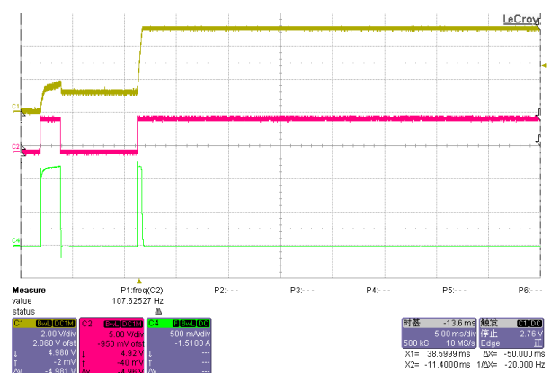
1 Ohm-load to No-load VIN=5V, RILIM=20K CH1: Output Voltage; CH2: n FAULT pin Voltage CH4: Input Current
