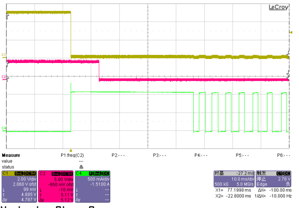
No-load to Short-Circuit VIN=5V, RILIM=20K CH1: Output Voltage; CH2: n FAULT pin Voltage; CH4: Input Current
