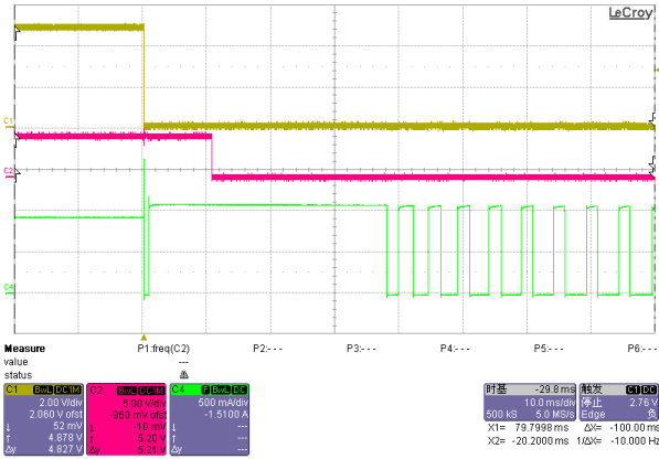
Full Load to Short-Circuit VIN=5V, RILIM=20K CH1: Output Voltage; CH2: n Fault pin Voltage; CH4: Input Current
