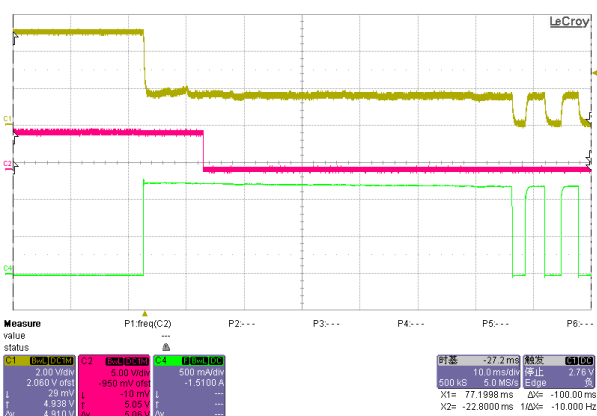
No-load to 1 Ohm-load VIN=5V, RILIM=20K CH1: Output Voltage; CH2: n FAULT pin Voltage CH4: Input Current
