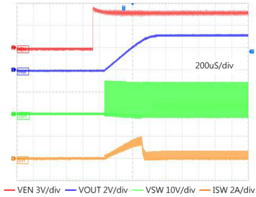
Turn On Waveform
