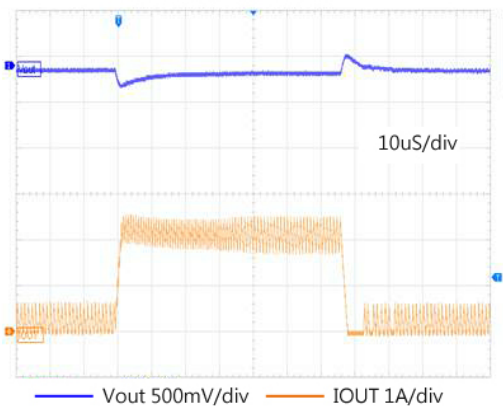
3.3V 0.1-2A Transient Response
