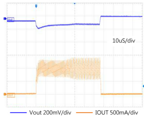
3.3V 0-1A Transient Response
