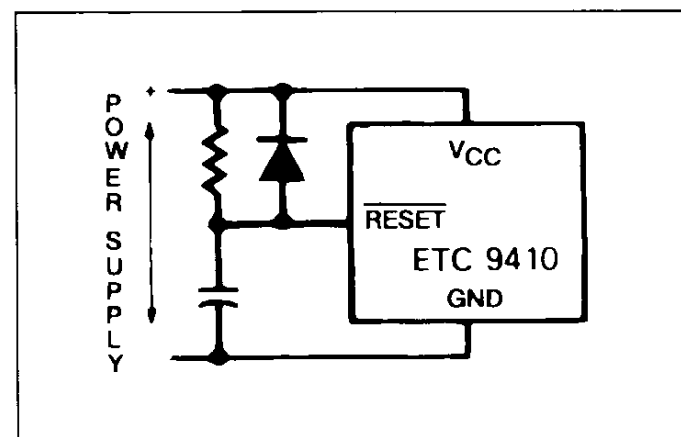
Figure 5 : Power-up Clear Circuit.
