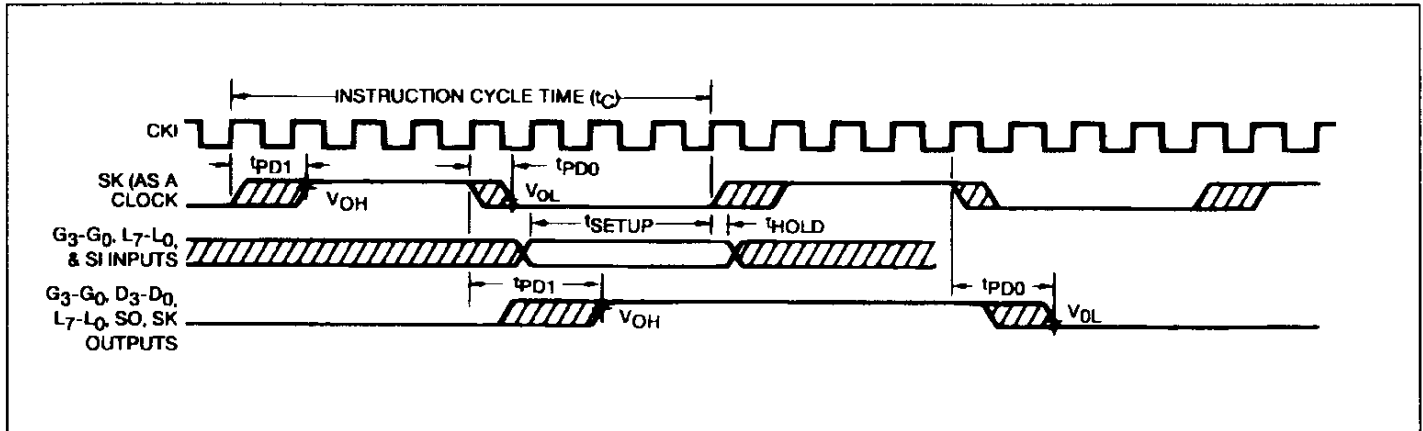
Figure 3 : Input/output Timing Diagrams (divide-by-8 mode).
