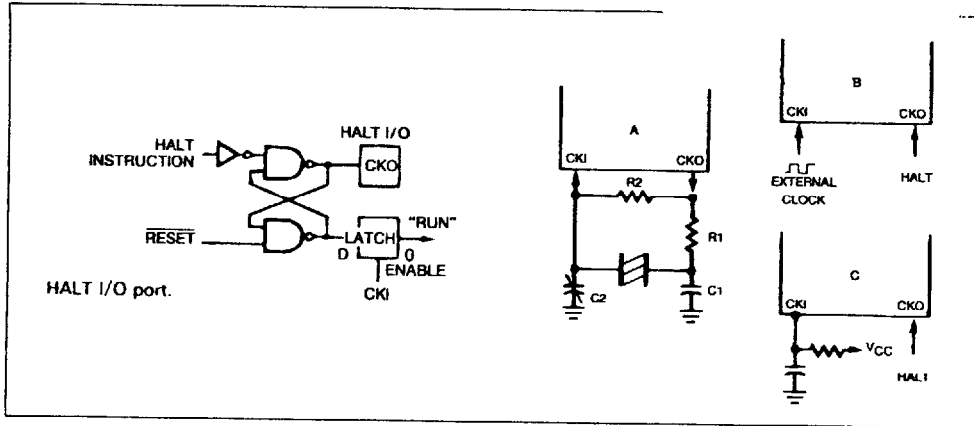
Figure 6 : ETC9410C Oscillator.
