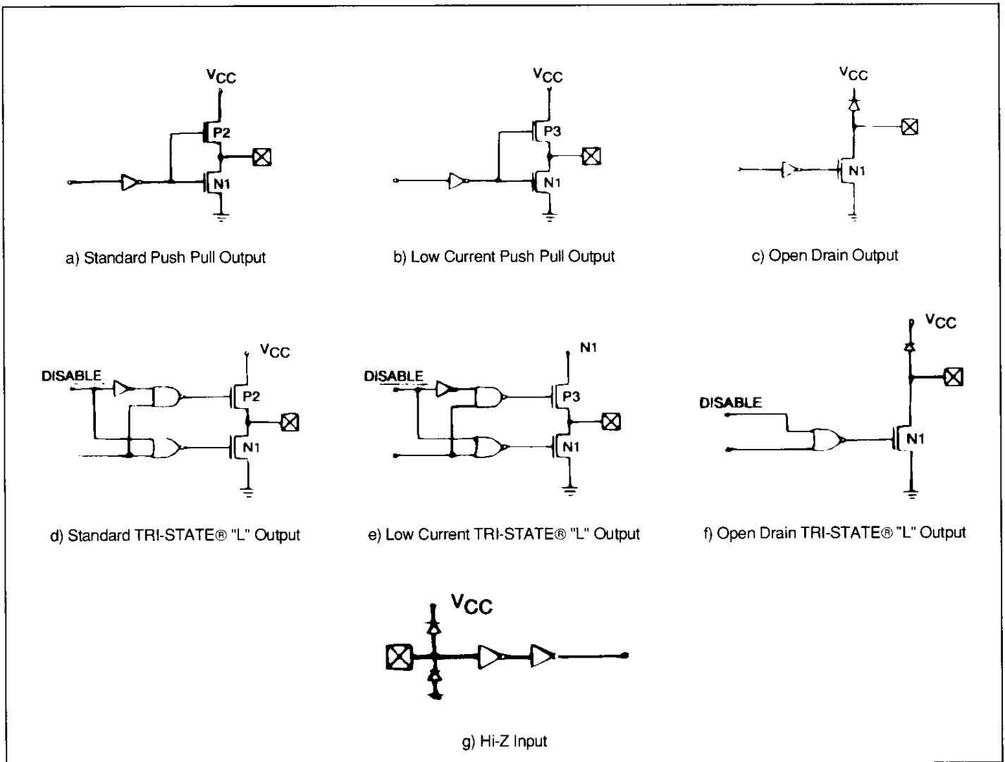
Figure 7 : Input and Output Configurations.
