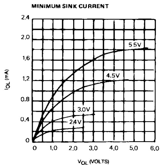
Figure 8 : Input/output Characteristics.
