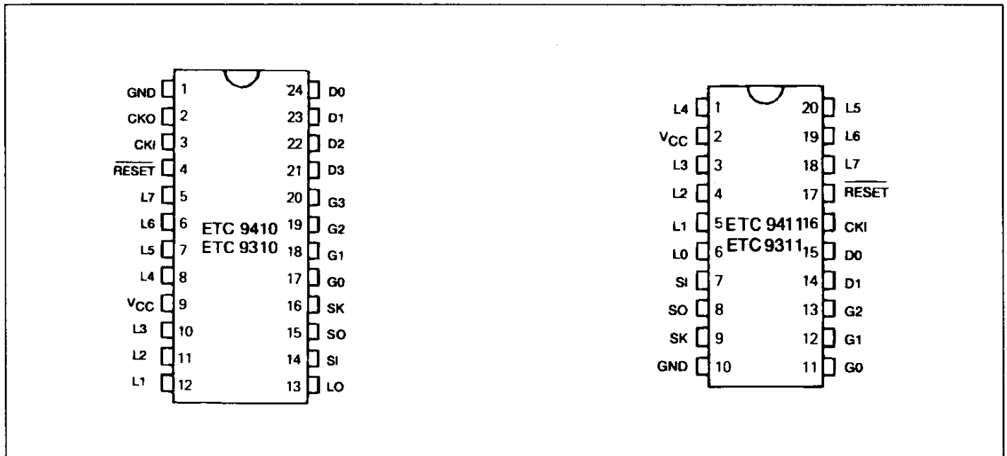
Figure 2 : Pin Connections.
