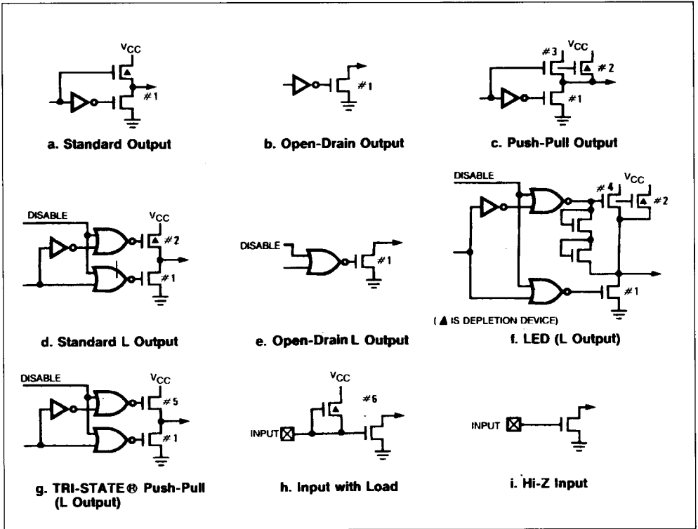
Figure 5 : Output Configurations.
