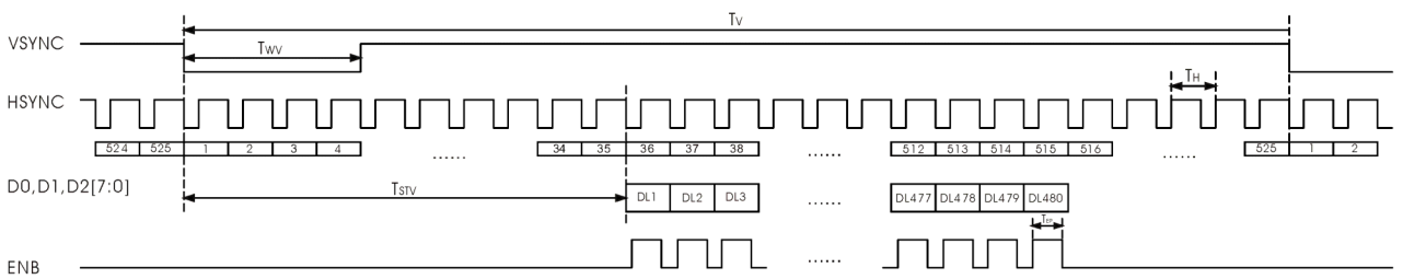
VERTICAL TIMING
