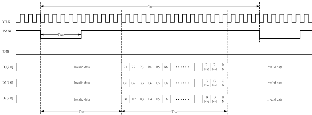
HORIZONTAL TIMING
