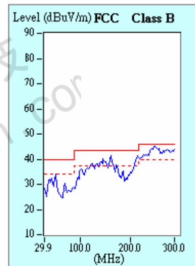
Figure29. EMI Test and FCC Limits
