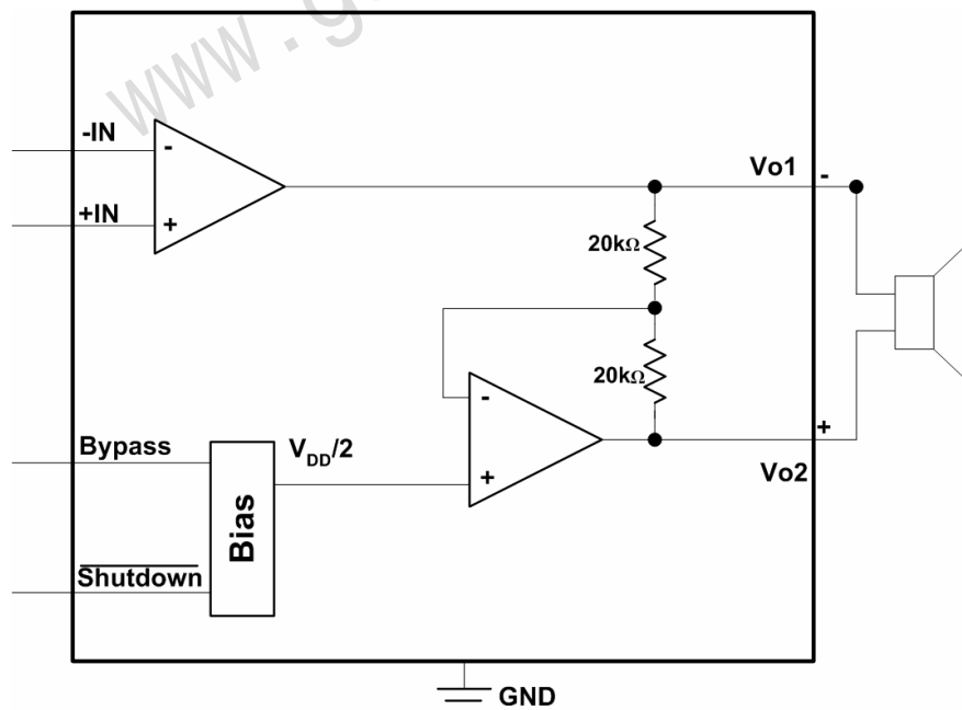
Figure1. Block Diagram
