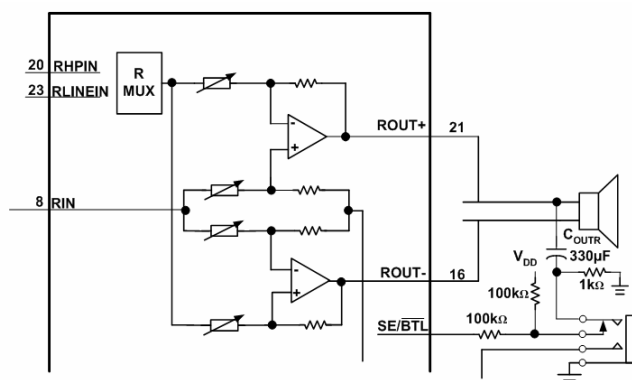
Figure 41. Resistor Divider Network Circuit
