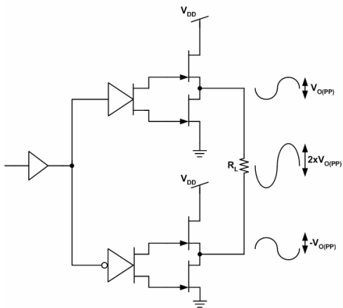
Figure 39. Bridge-Tied Load Configuration
