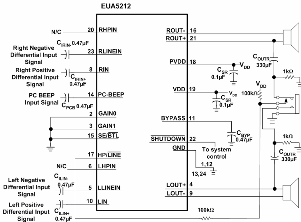
Figure 2. Application circuit using differential input
