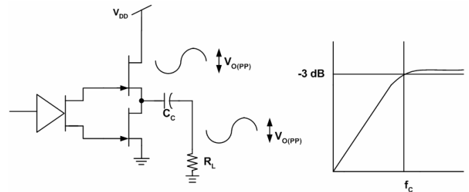
Figure 40. Single-Ended Configuration and Frequency Response
