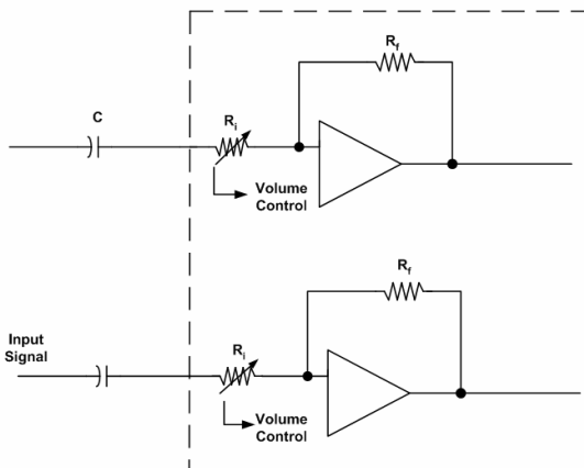
Figure 38. Input Resistor
