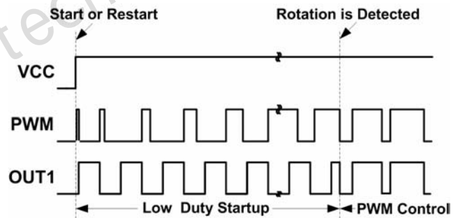
Figure 9. Low Duty Startup Function
