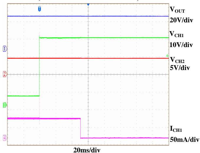
Protection of Inductor Short
