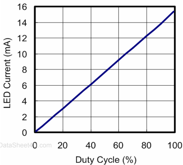
Duty Cycle vs LED Current ILED 1-4=15.5mA
