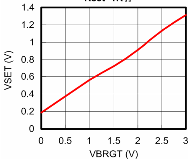
V set vs V BRGT Rset=1KΩ
