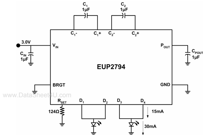
Figure 5. Two Parallel Connected LEDs
