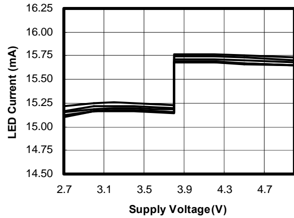
LED Current Matching vs. Supply Voltage ( R_{set}=7.5K\Omega , V_{LED}=3.6V )
