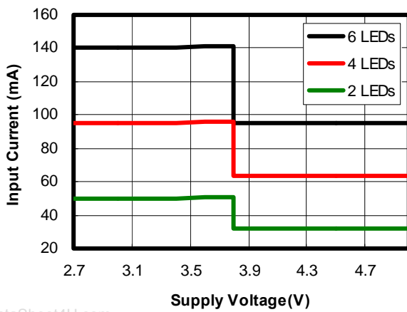
Input Current vs. Supply Voltage ( R_{set}=7.5K\Omega , V_{LED}=3.6V )
