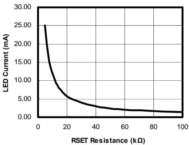
LED Current vs RSET
