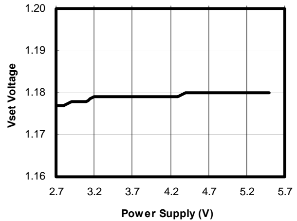
Vset vs Power Supply
