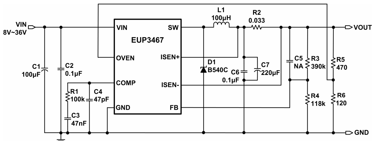
Figure 1. Application Circuit
