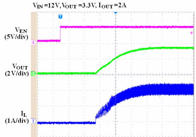
Times (100us/div)
