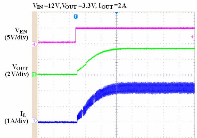
Times (4ms/div)
