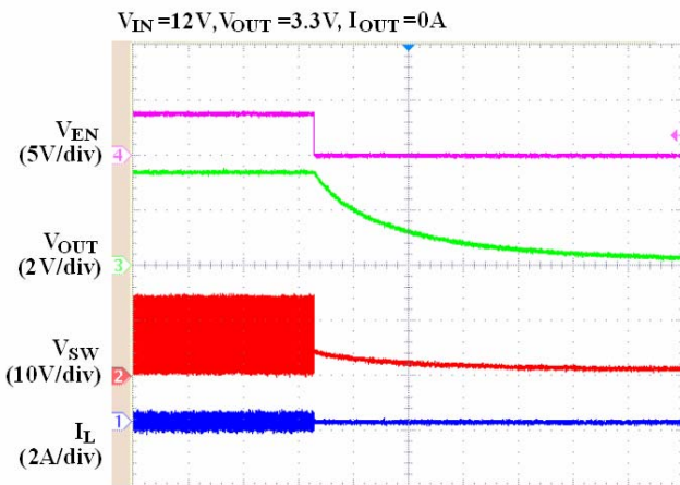
Times (400ms/div)
