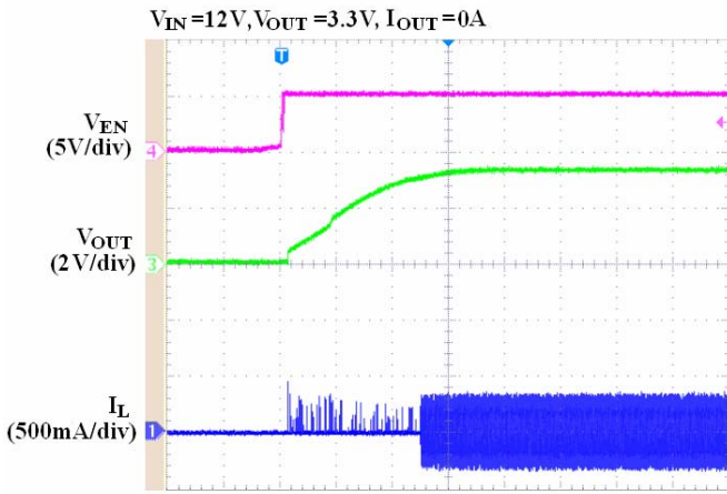
Times (4ms/div)
