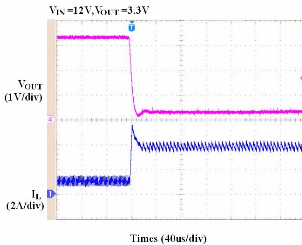
Short Circuit
