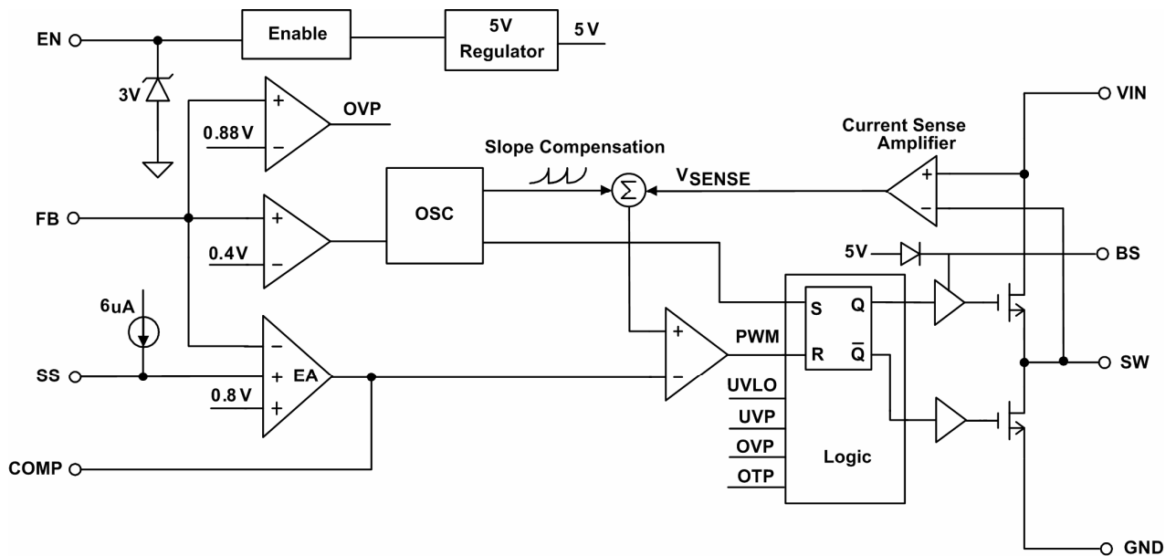
Figure 3. EUP3472 Functional Block Diagram
