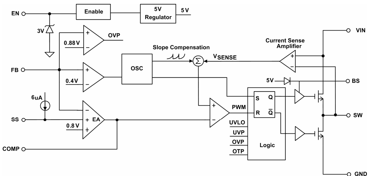
Figure 2. EUP3475A Functional Block Diagram
