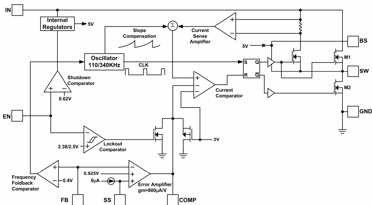
Figure 3.Functional Block Diagram
