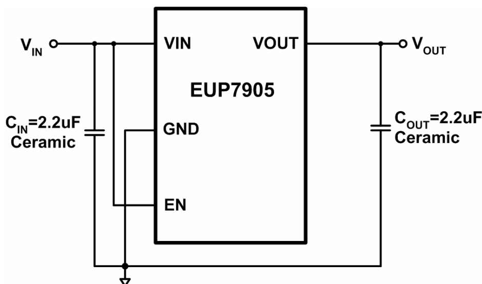
Figure. 1 Fixed Output
