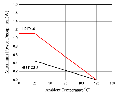
Figure 5. Power Dissipation for EUP7905 Packages
