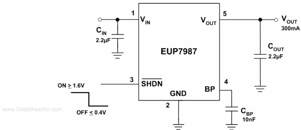
Figure2. Fixed-Voltage LDO Regulator
