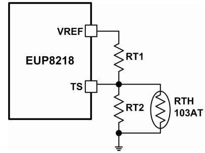
Figure 7. TS Resistor Network
