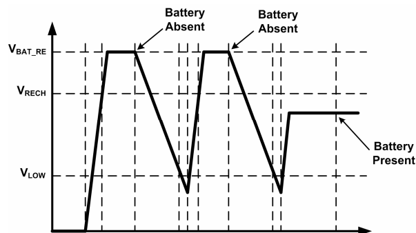
Figure 5. Battery Detect Timing Diagram
