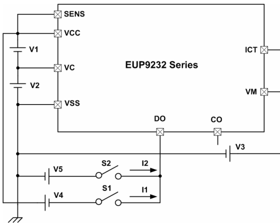
Test Circuit 3
