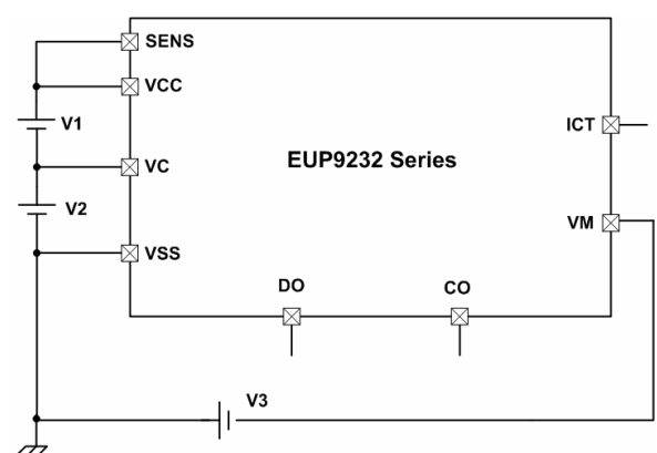
Test Circuit 6
