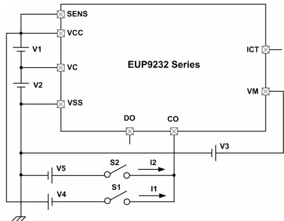
Test Circuit 4
