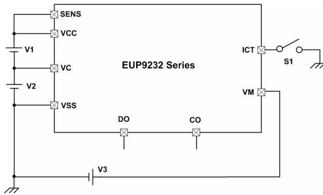
Test Circuit 1
