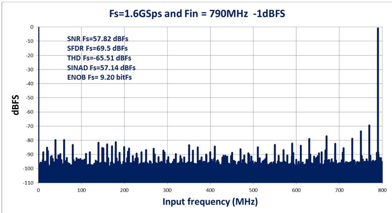
Figure 26 FFT at 1.6GSps and F_{in} = 790\text{MHz} / -1dBFS
