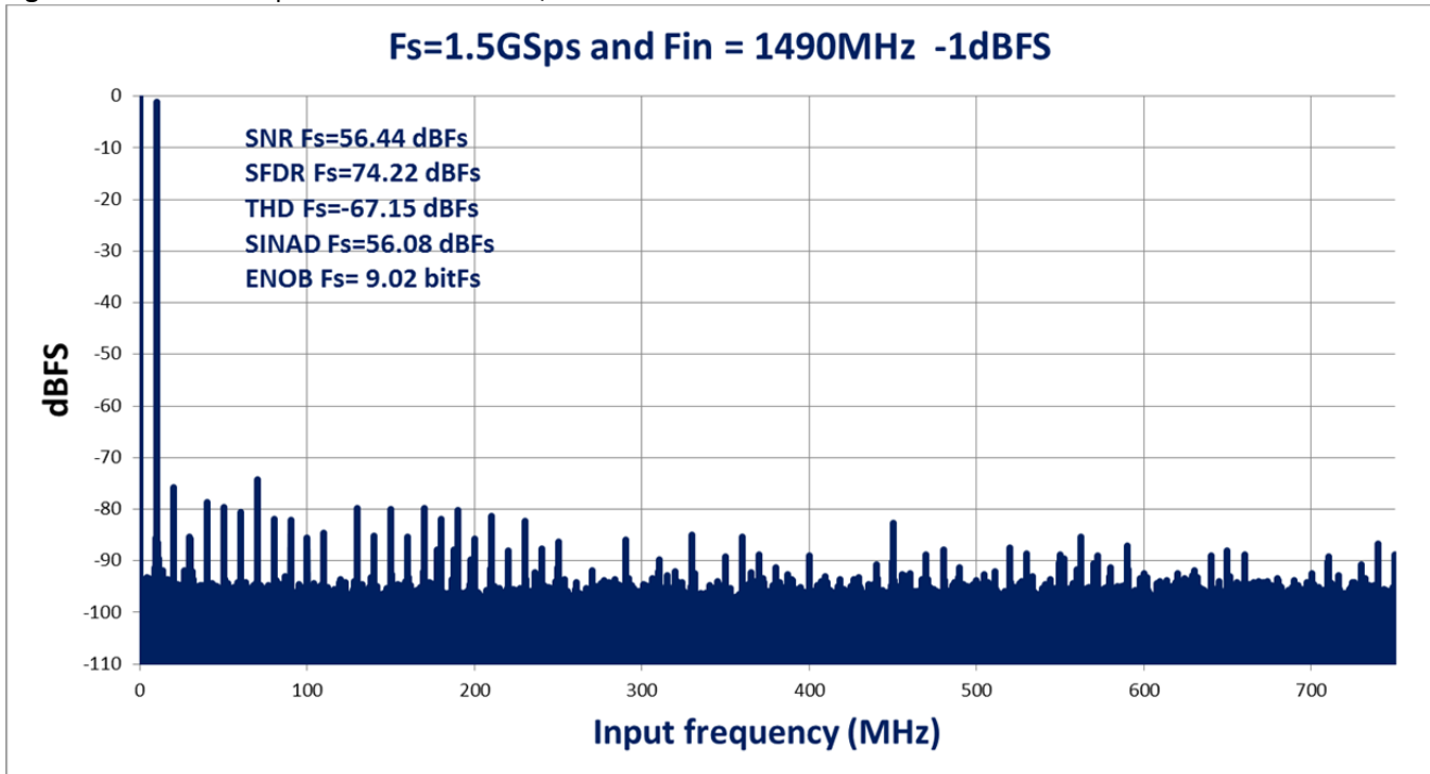
Figure 27: FFT at 1.5GSps and F_{in} = 1490\text{MHz} / -1dBFS
