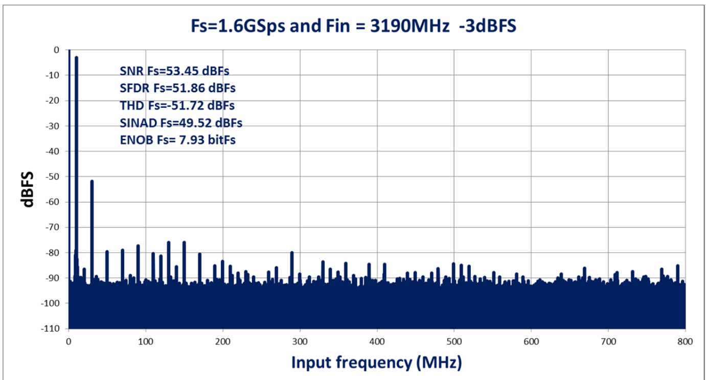
Figure 32 FFT at 1.6GSps and F_{in} = 3190\text{MHz} / -3dBFS
