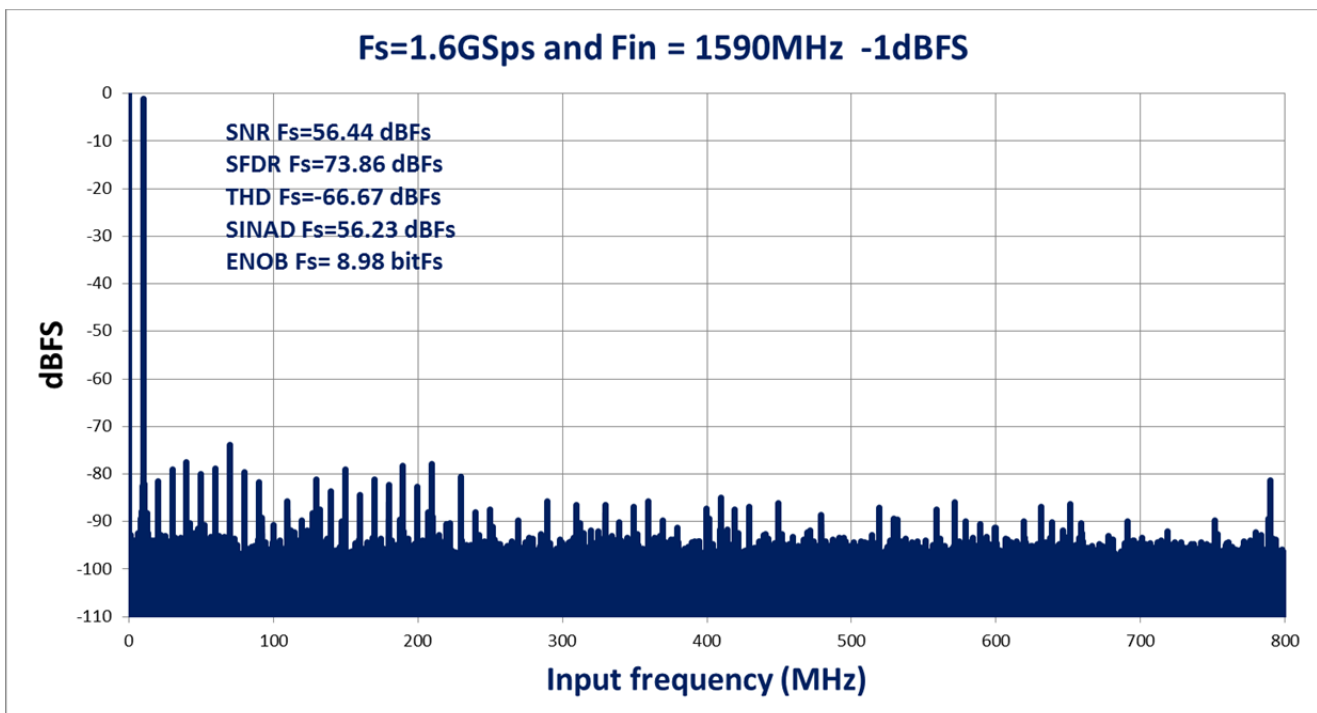
Figure 28 FFT at 1.6GSps and F_{in} = 1590\text{MHz} / -1dBFS
