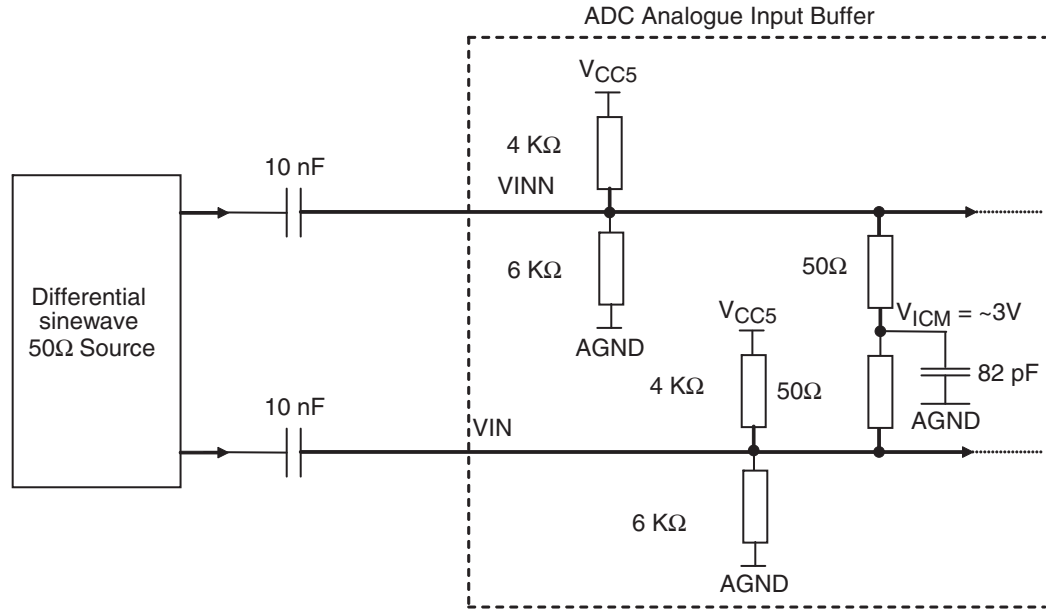
Figure 7-3. Differential Analogue Input Implementation (AC Coupled)
