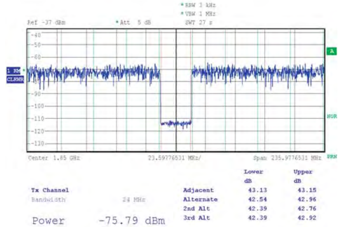
Figure 7-45. NPR in second Nyquist Zone, 1520 MHz to 2200 MHz noise pattern with a 25 MHz notch centered on 1850 MHz, RF Mode
