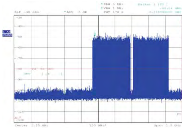
Figure 7-46. NPR in second Nyquist Zone, 2200 MHz to 2880 MHz Noise Pattern with a 25 MHz Notch centered on 2550 MHz, RF Mode
