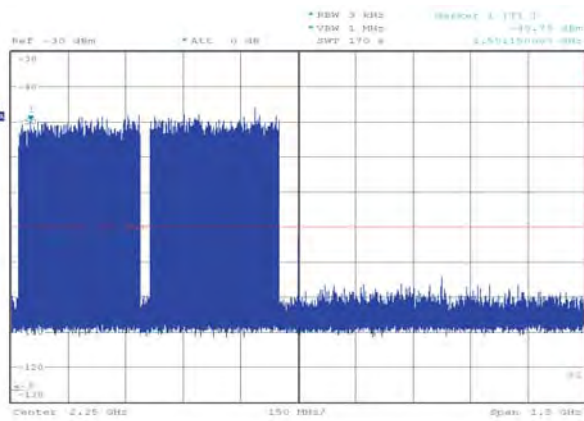
Figure 7-45. NPR in second Nyquist Zone, 1520 MHz to 2200 MHz noise pattern with a 25 MHz notch centered on 1850 MHz, RF Mode
