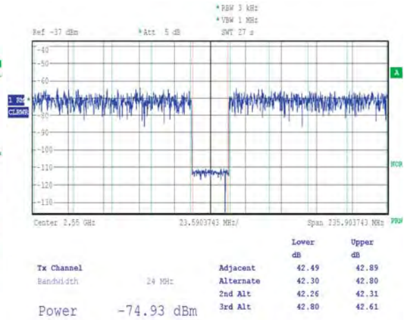
Figure 7-46. NPR in second Nyquist Zone, 2200 MHz to 2880 MHz Noise Pattern with a 25 MHz Notch centered on 2550 MHz, RF Mode
