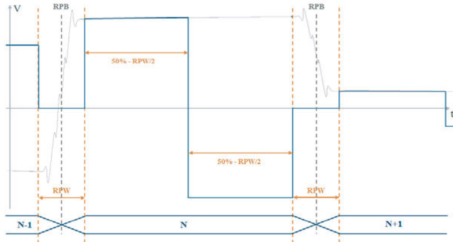
Figure 21. DAC output in RF mode and time domain when RPB and RPW are optimum
