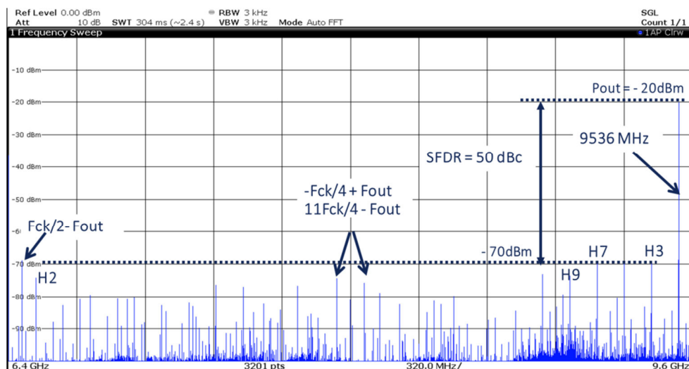
Figure 54. Typical SFDR spectrum in RF mode with F_{out} = 9536 \text{ MHz} ( 3^{\text{rd}} Nyquist), MUX4:1, F_s = 6.4 \text{ GSps} , SFDR = 50 dBc
