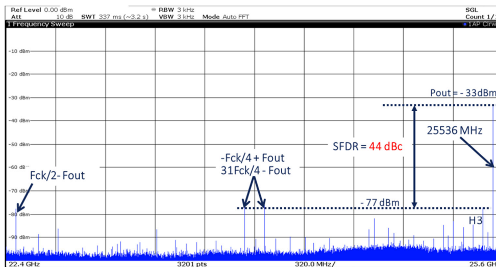
Figure 59 Typical SFDR spectrum in RF mode with F_{out} = 25536 \text{ MHz} (8 th Nyquist), MUX4:1, F_s = 6.4 \text{ GSps} , SFDR = 44 dBc
