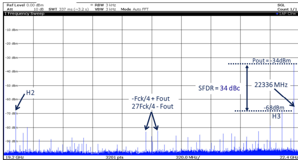
Figure 58 Typical SFDR spectrum in RF mode with F_{out} = 22336 \text{ MHz} (7 th Nyquist), MUX4:1, F_s = 6.4 \text{ GSps} , SFDR = 34 dBc
