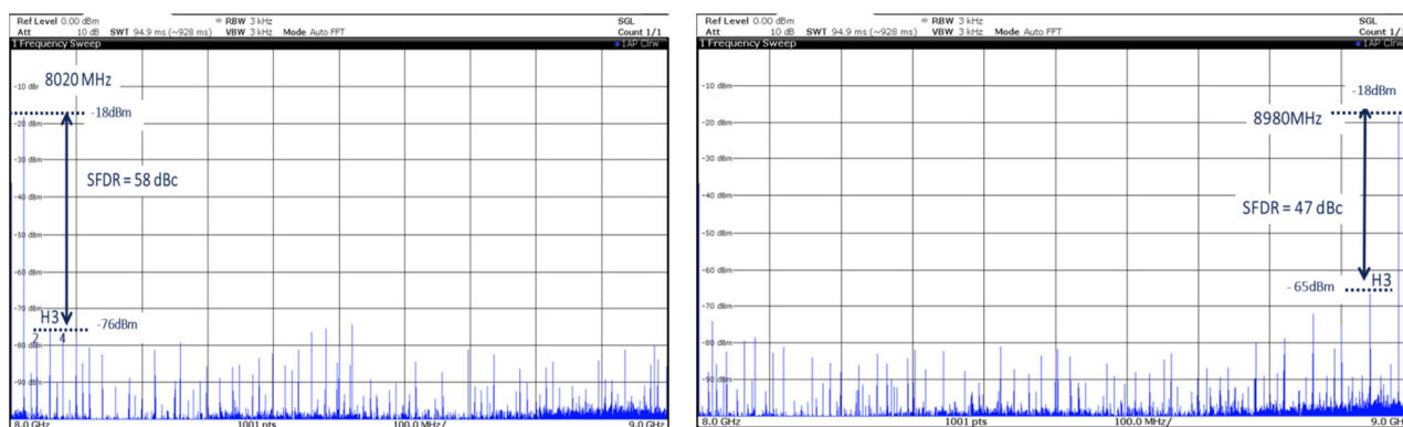
Figure 70. Typical SFDR spectrum in RF mode in IUCM4 Mode in NZ9 ( F_{out} = 8020 MHz) and ( F_{out} = 8980 MHz), F_s = 8.0 GSps
