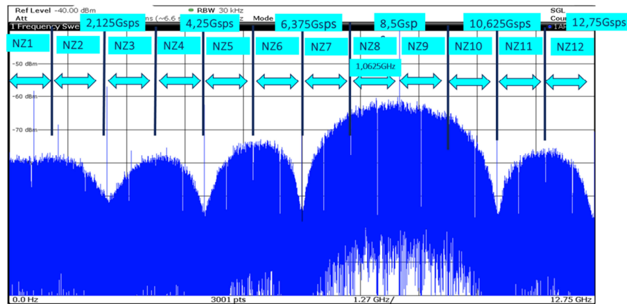
Figure 119. NPR at 8.5 Gsps in IUCM2 in RF mode in 4 th Nyquist and 5 th Nyquist Zone
