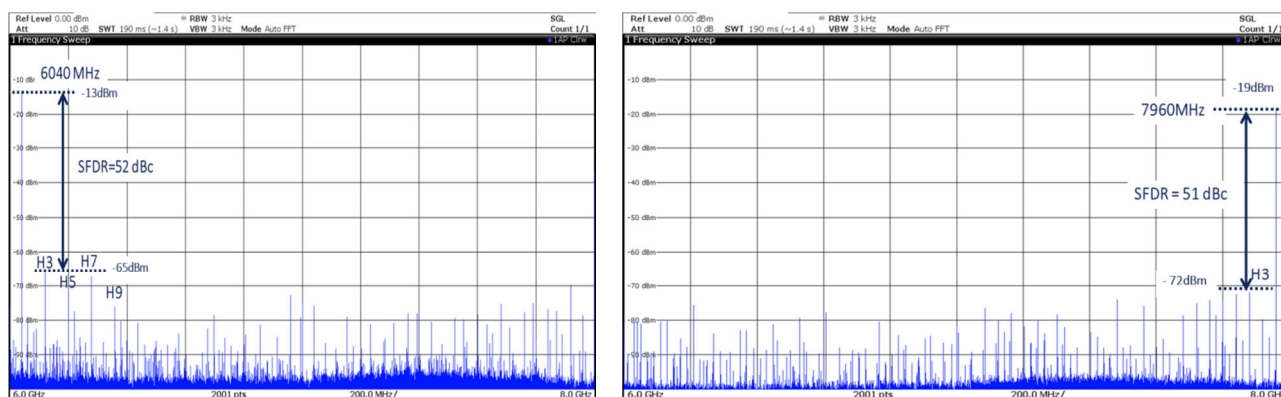
Figure 67. Typical SFDR spectrum in RF mode in IUCM2 Mode in NZ4 ( F_{out} = 6040 \text{ MHz} ) and ( F_{out} = 7960 \text{ MHz} ), F_s = 8.0 \text{ GSpS}
