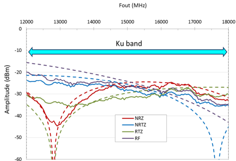
Figure 43. Pout vs Fout @ 6.4 GSps from 12 GHz to 18 GHz vs modes (Ku-Band)
