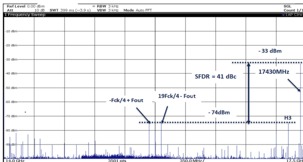
Figure 64. Typical SFDR spectrum in RF mode with F_{out} = 17430 \text{ MHz} ( 5^{\text{th}} Nyquist), MUX4:1, F_s = 7.0 \text{ GSps} , SFDR = 41 dBc
