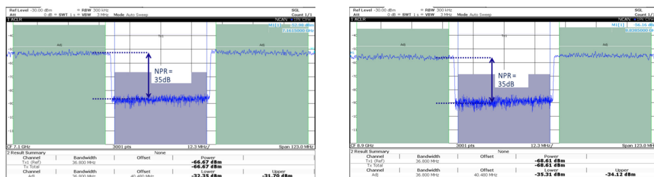
Figure 115. NPR at 8.0 Gsps in IUCM2 in RF mode in 4 th Nyquist and 5 th Nyquist Zone
