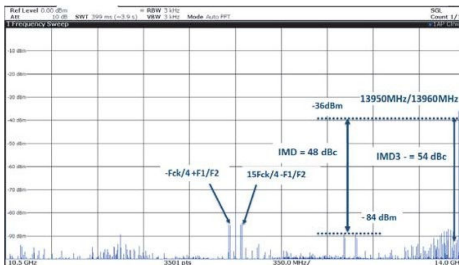
Figure 93. Typical Dual-tone spectrum in NRTZ mode with Fout1,Fout2 = 13950 MHz,13960 MHz, (4 th Nyquist), MUX4:1, Fs = 7.0 GSps, IMD3 - = 54 dBc, IMD full Nyquist = 48 dBc
