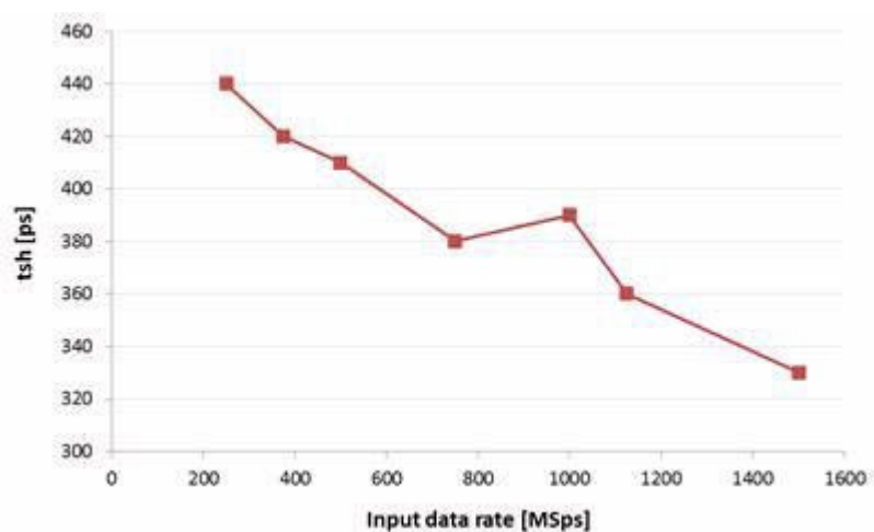
Figure 121. t_{SH} vs input data rate
