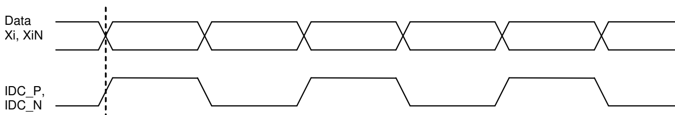
Figure 30. IDC timing vs data input
