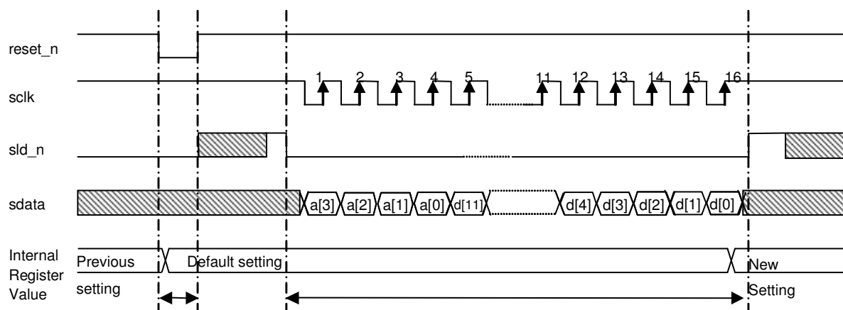
Figure 34. 3WSI Timing Diagram
