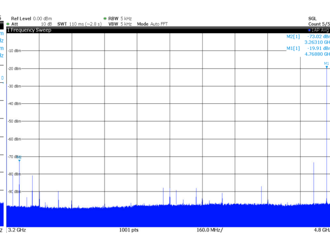
Figure 80. Typical SFDR spectrum in RF mode. Fout = 4768 MHz (3 rd Nyquist), MUX2:1, Fs = 3.2 GSps. SFDR = 53 dBc
