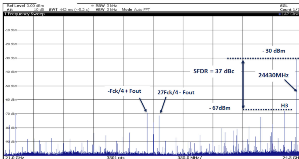
Figure 66. Typical SFDR spectrum in RF mode with F_{out} = 24430 \text{ MHz} (7 th Nyquist), MUX4:1, F_s = 7.0 \text{ GSpS} , SFDR = 37 dBc
