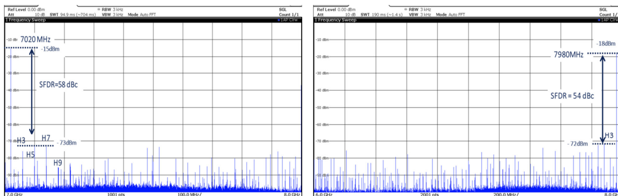
Figure 69. Typical SFDR spectrum in RF mode in IUCM4 Mode in NZ8 ( F_{out} = 7020 MHz) and ( F_{out} = 7980 MHz), F_s = 8.0 GSps
