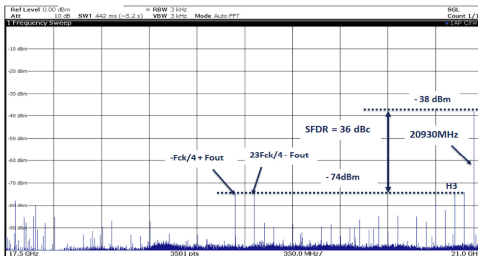
Figure 65. Typical SFDR spectrum in RF mode with F_{out} = 20930 \text{ MHz} ( 6^{\text{th}} Nyquist), MUX4:1, F_s = 7.0 \text{ GSps} , SFDR = 36 dBc
