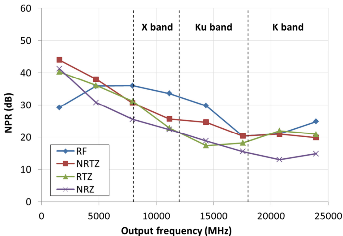
Figure 110. NPR vs Output Frequency from 1 GHz to 23 GHz, vs modes (covering X-Band, Ku-Band, K-Band)
