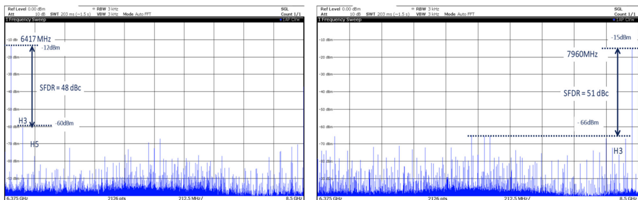
Figure 71. Typical SFDR spectrum in RF mode in IUCM2 Mode in NZ4 ( F_{out} = 6417 MHz) and ( F_{out} = 7960 MHz), F_s = 8.5 GSps
