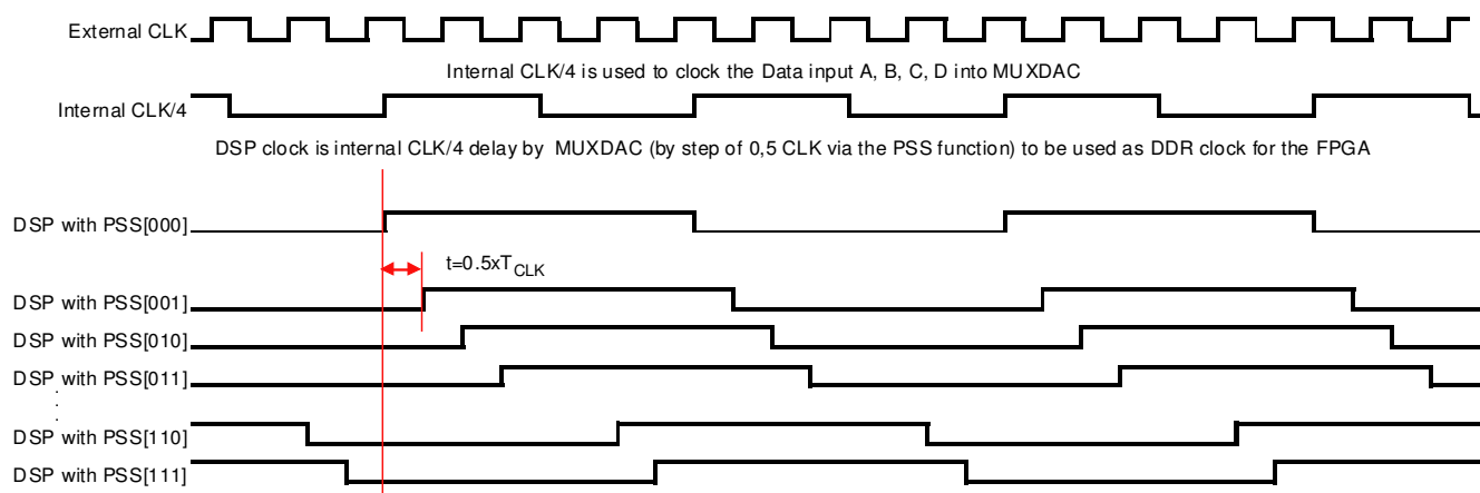
Figure 22. PSS timing diagram for 4:1 MUX, OCDS = 0
