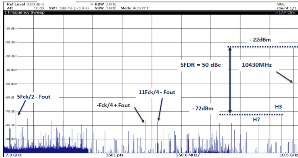
Figure 62. Typical SFDR spectrum in RF mode with F_{out} = 10430 \text{ MHz} ( 3^{\text{rd}} Nyquist), MUX4:1, F_s = 7.0 \text{ GSps} , SFDR = 50 dBc
