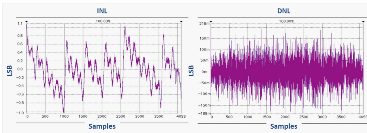
Figure 36. INL & DNL measurements at F_{out} = 100\text{ kHz} , F_{clock} = 3\text{ GHz}
