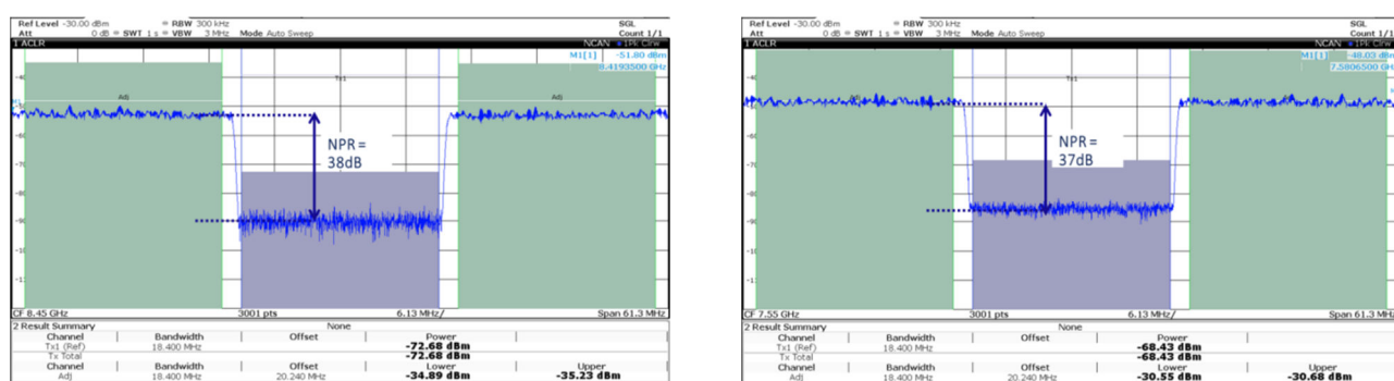
Figure 116. NPR at 8.0 Gsps in IUCM4 in RF mode in 8 th Nyquist and 9 th Nyquist Zone
