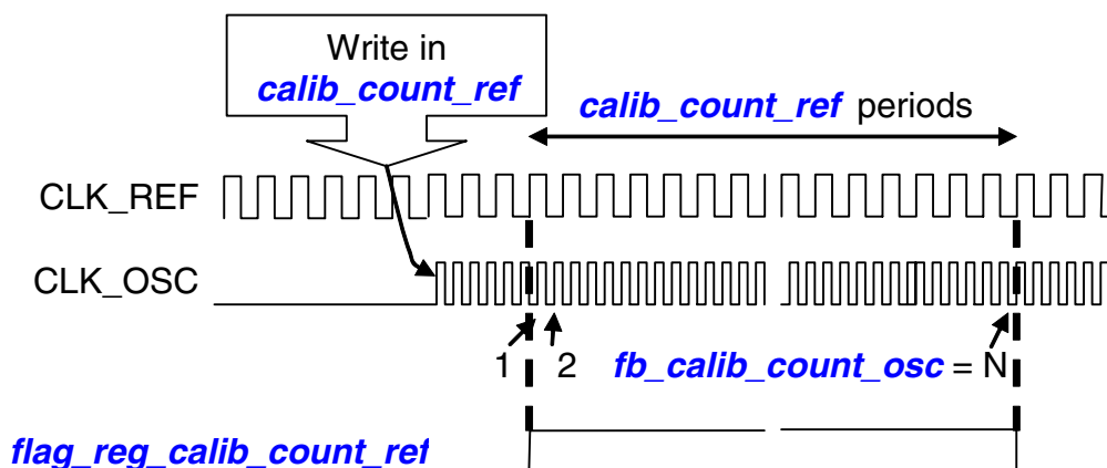
Figure 15-4. Oscillator calibration
