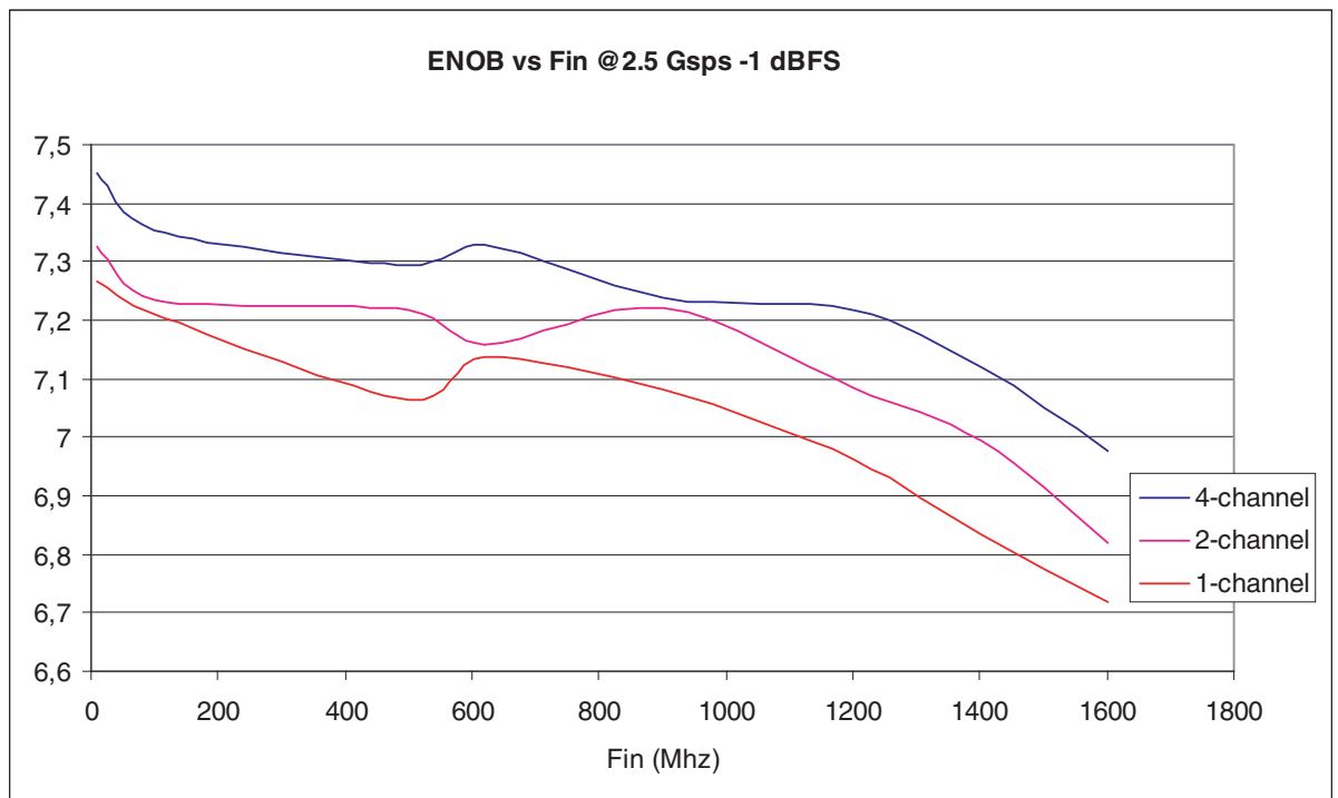
Figure 4-3. ENOB vs Fin
