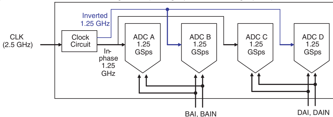
Figure 2-5. 2-channel Mode Configuration (Analog Input B and Analog Input D)
