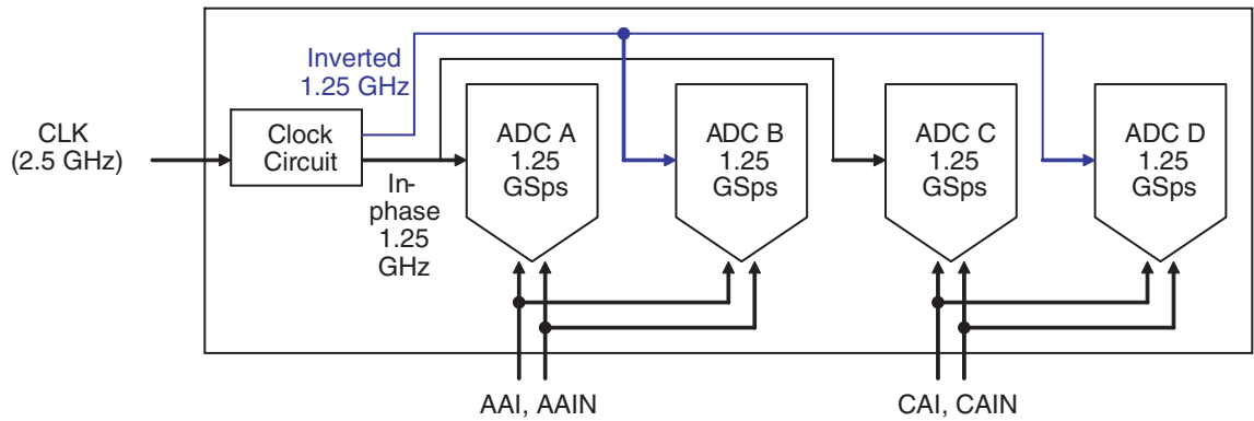
Figure 2-2. 2-channel Mode Configuration (Analog Input A and Analog Input C)
