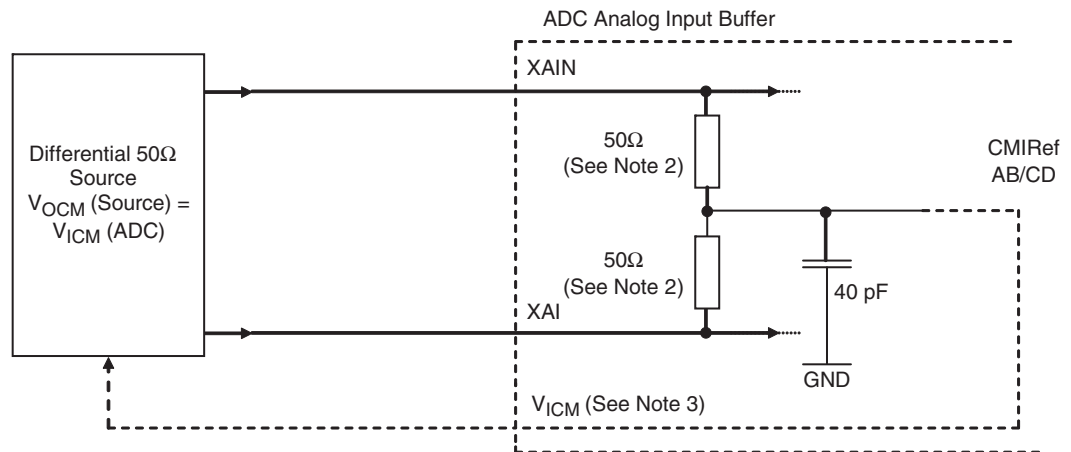
Figure 7-4. Differential analog input implementation (DC coupled)
