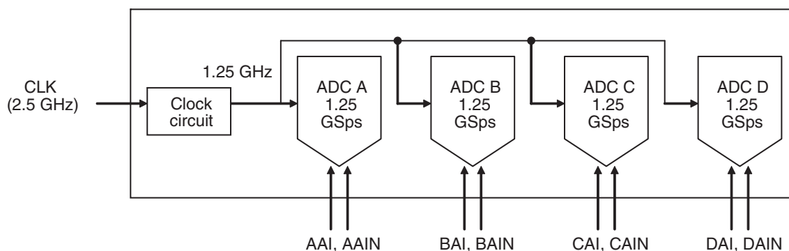
Figure 2-1. 4-channel Mode Configuration
