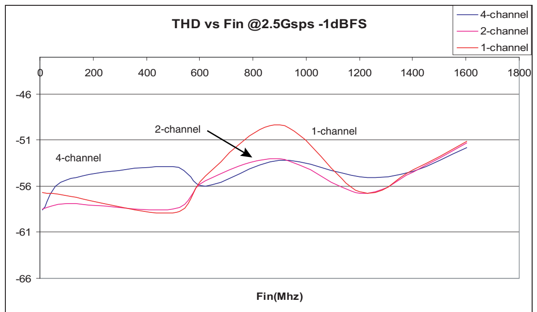
Figure 4-5. THD vs Fin
