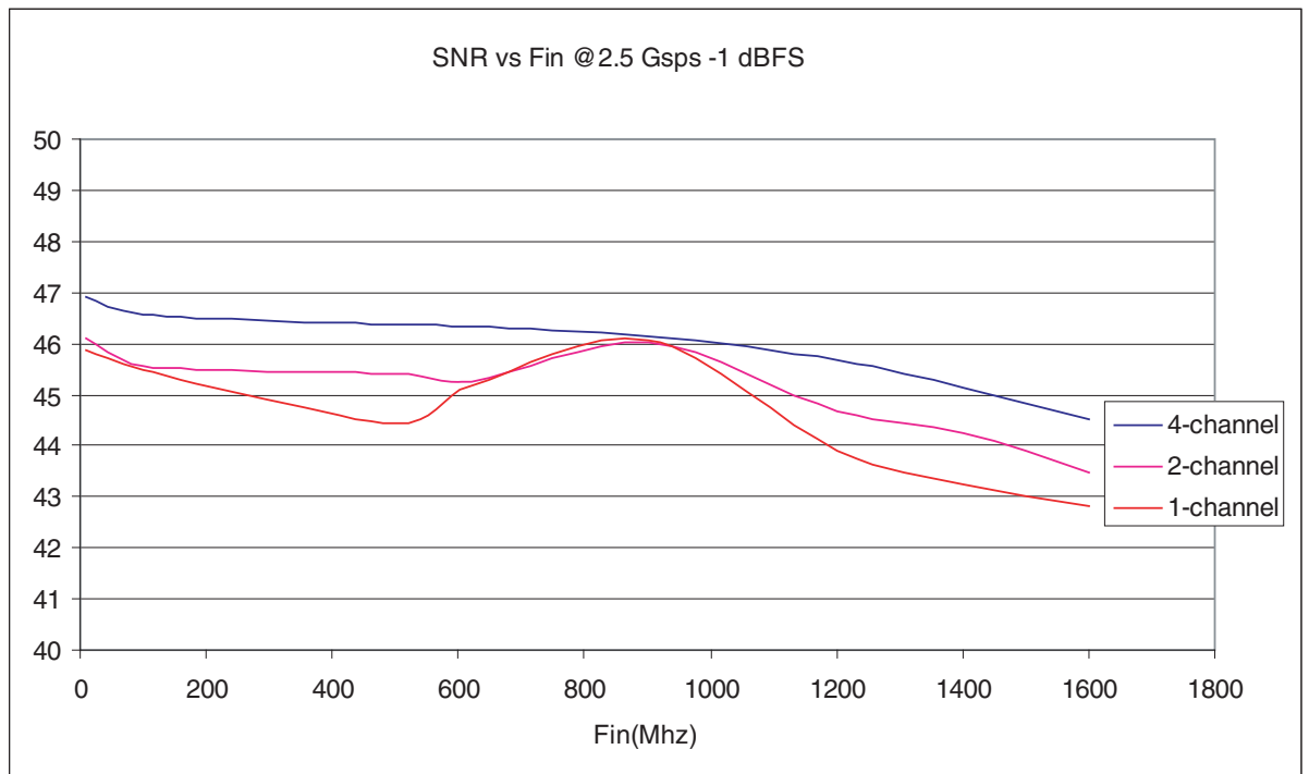
Figure 4-4. SNR vs Fin
