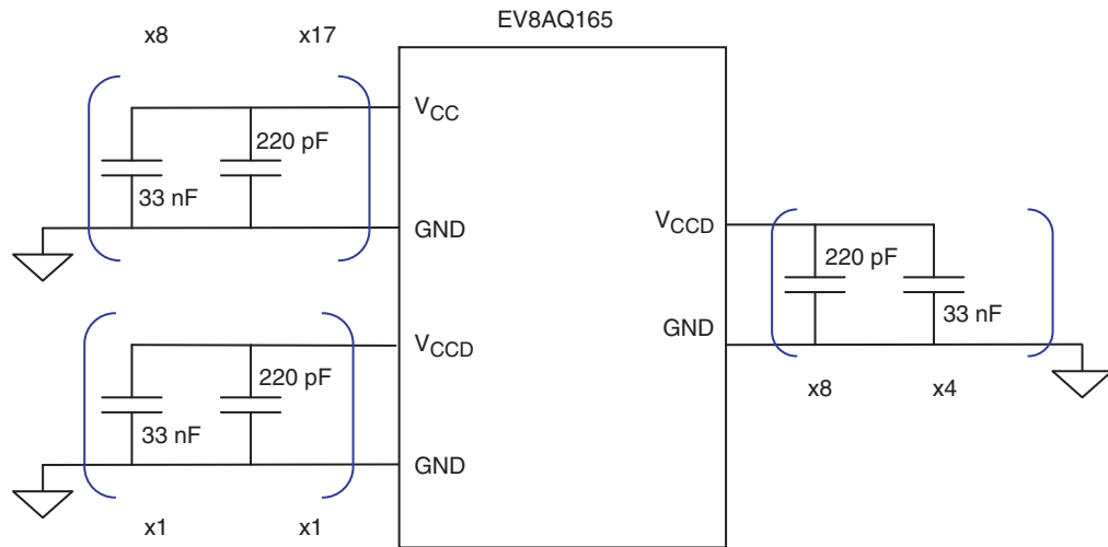
Figure 7-2. EV8AQ165A Power Supplies Bypassing Scheme
