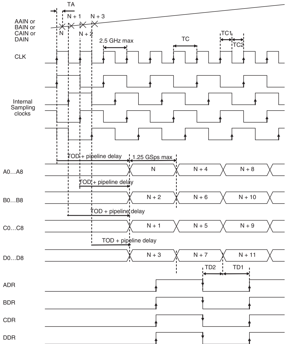
Figure 3-3. ADC Timing in 1-Channel Mode
