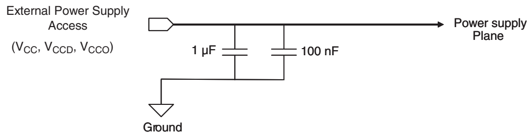
Figure 7-1. EV8AQ165A Power supplies Decoupling and grounding Scheme
