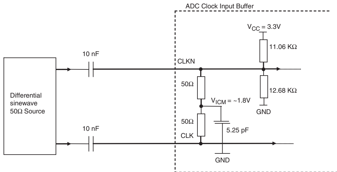
Figure 7-5. Differential Clock Input Implementation (AC coupled)
