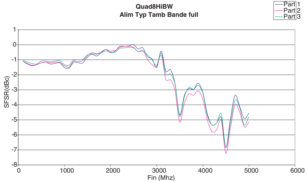
Figure 4-1. Full Power Input Bandwidth (-1 dBFS input, 1-channel mode, F_c = 2.5\text{GHz} , Full bandwidth setting )
