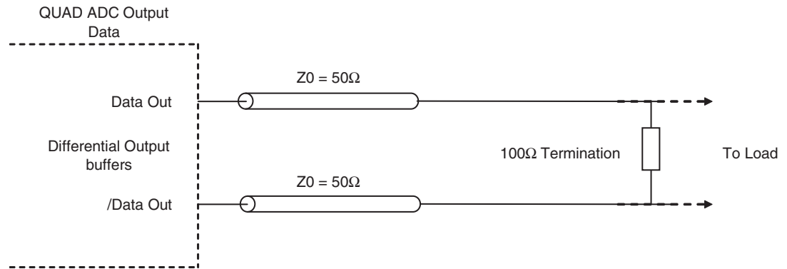
Figure 7-6. Differential Digital Outputs Terminations (100Ω LVDS)
