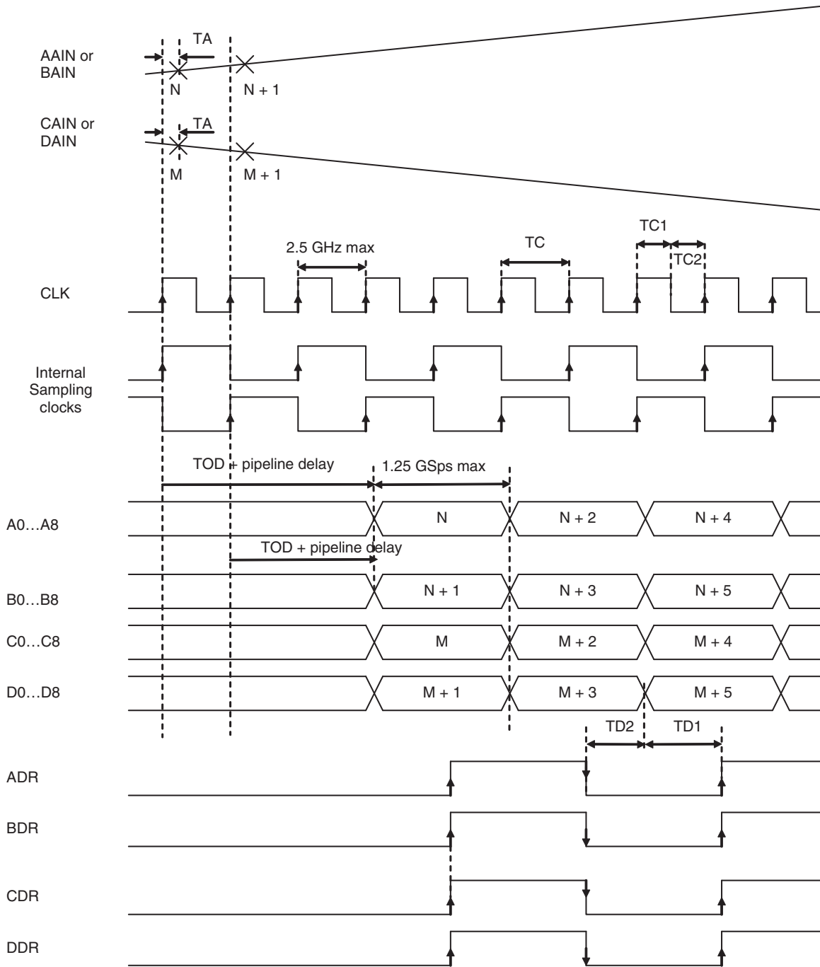
Figure 3-2. ADC Timing in 2-Channel Mode
