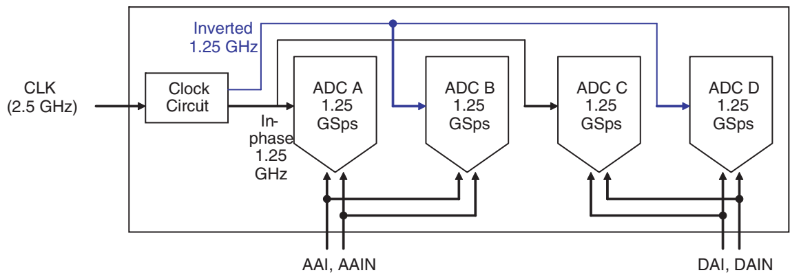
Figure 2-3. 2-channel Mode Configuration (Analog Input A and Analog Input D)
