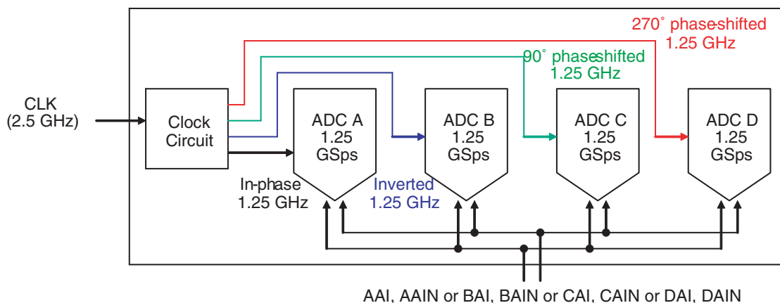
Figure 2-6. 1-channel Mode Configuration
