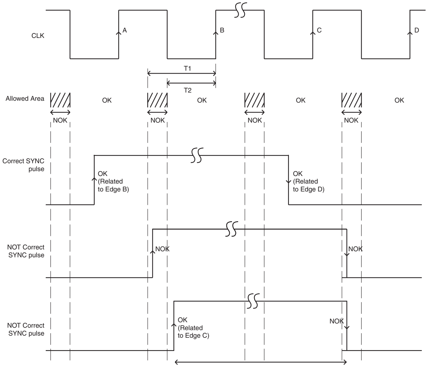
Figure 6-3. ADC SYNC Timing Condition
