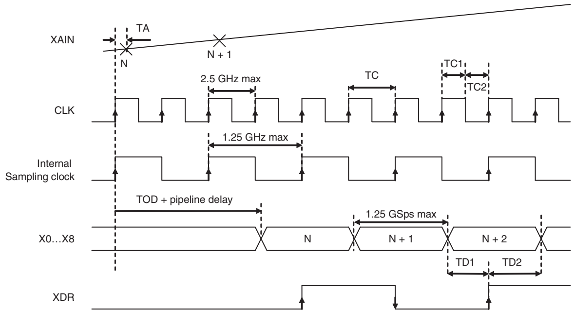
Figure 3-1. ADC Timing in 4-Channel Mode
