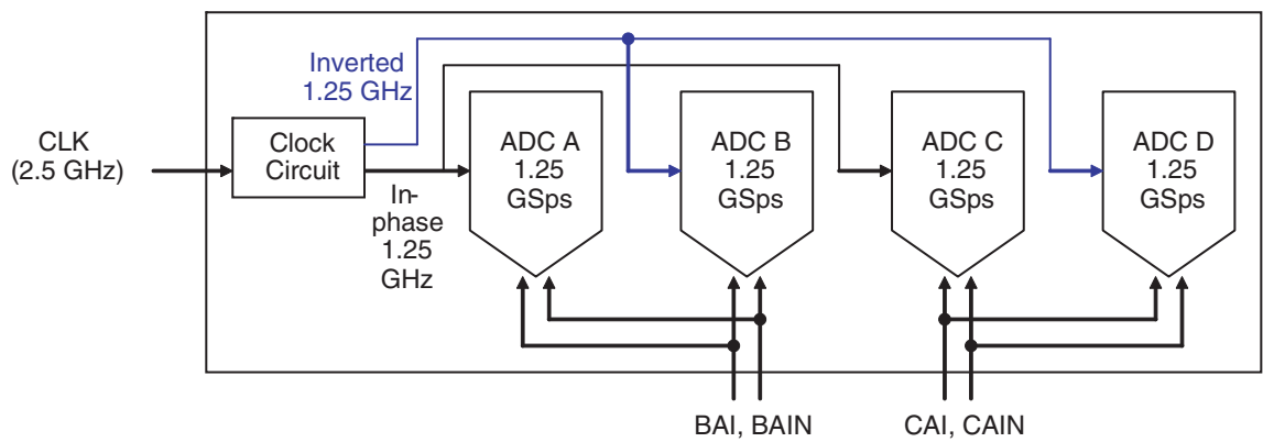
Figure 2-4. 2-channel Mode Configuration (Analog Input B and Analog Input C)
