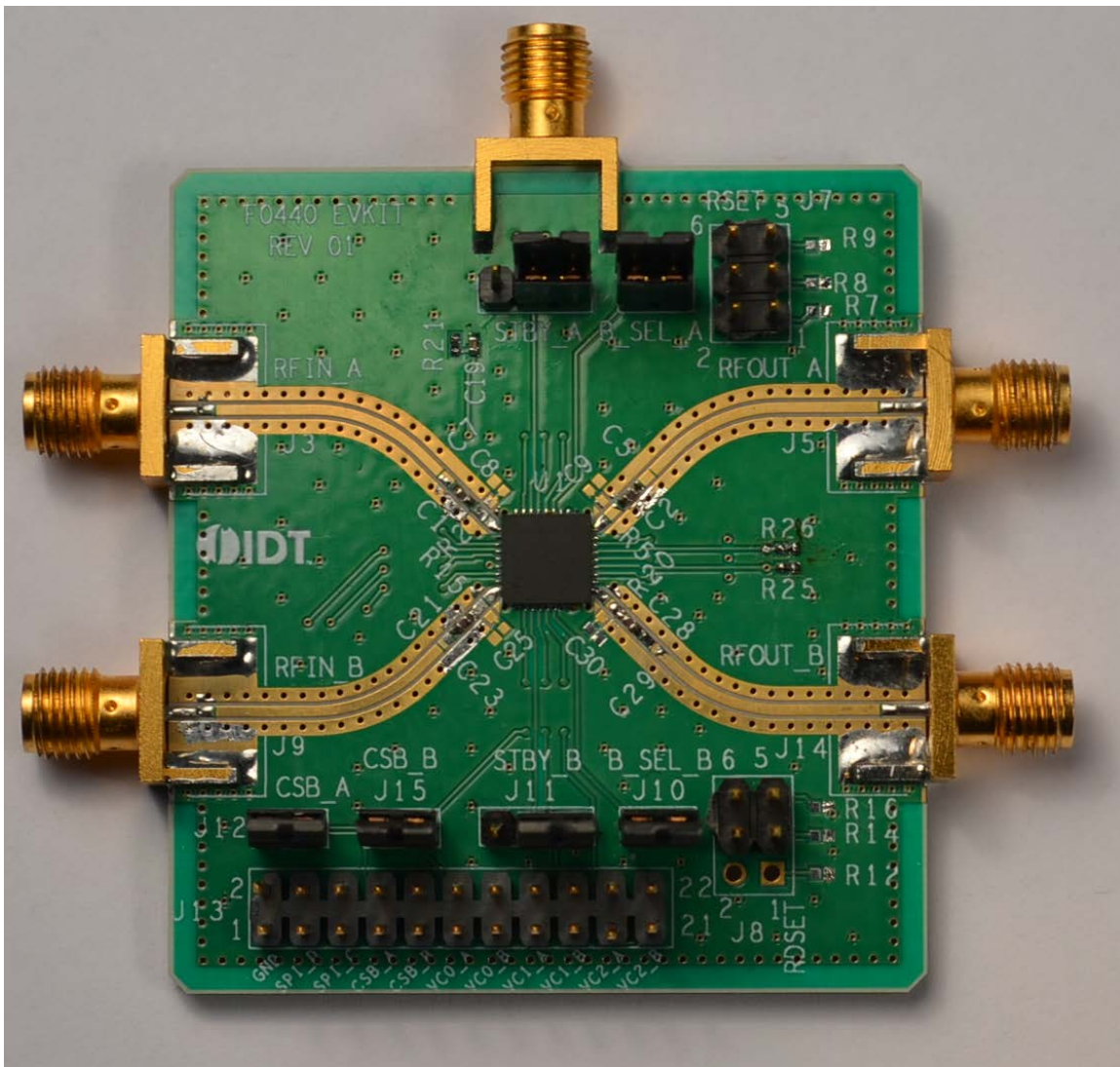
Figure 42. Top View
