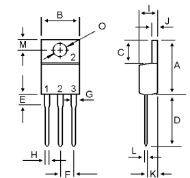
TO-220AB
