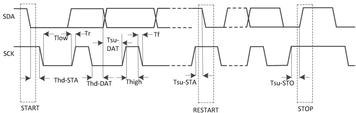
Figure 5-22 TWI Timing
