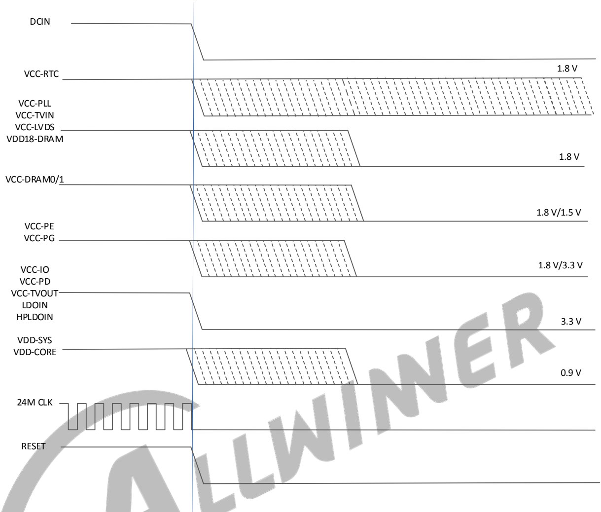
Figure 5-29 Power-Off Timing
