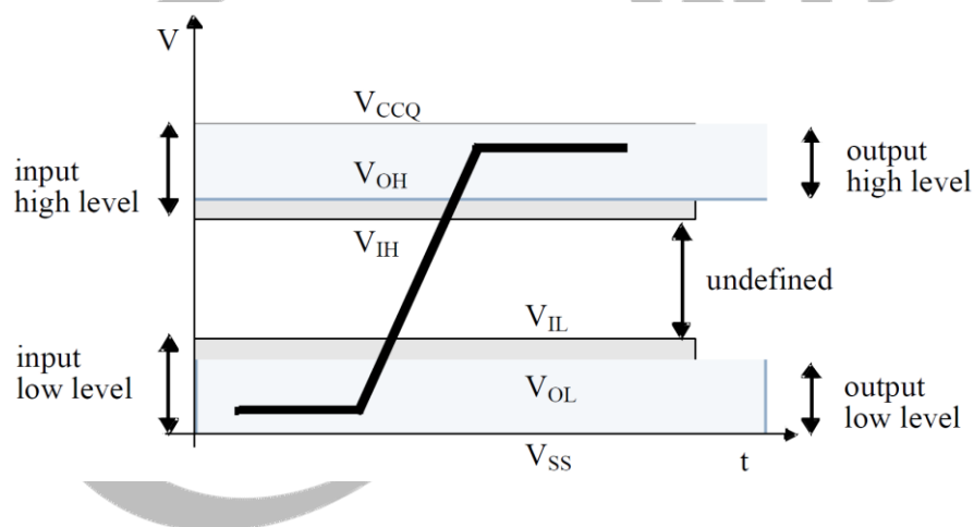
Figure 5-1 SDIO Voltage Waveform
