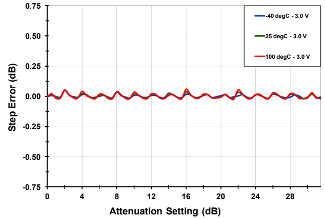
DNL [1900 MHz]
