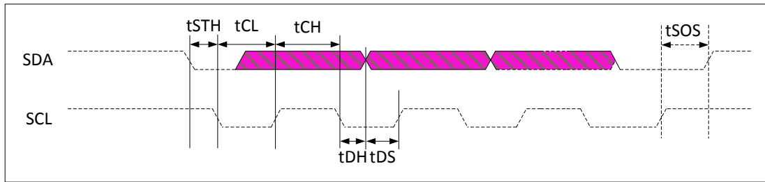
Figure 5-11. TWI Timing Diagram
