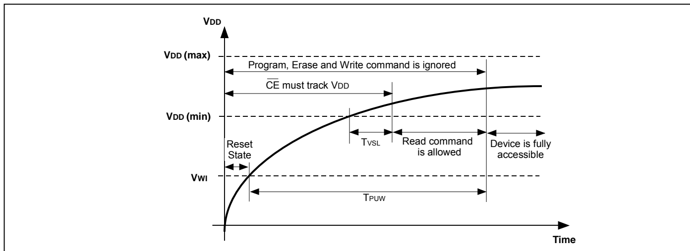
Figure 37: Power-Up Timing Diagram
