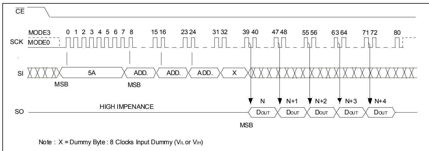
Figure 32: Read Serial Flash Discoverable Parameter (RDSFDP) Sequence
