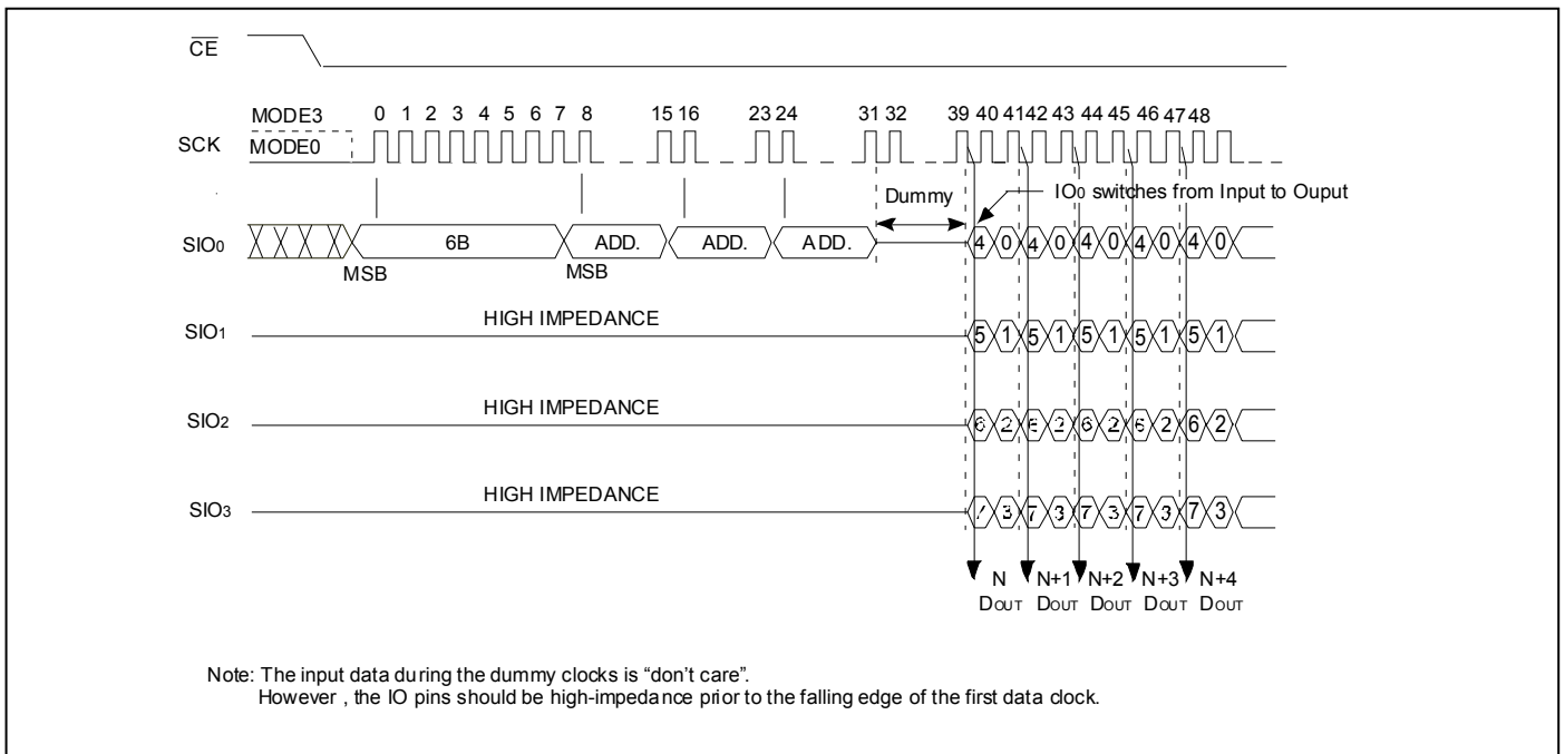
Figure 29: Fast Read Quad Output Sequence
