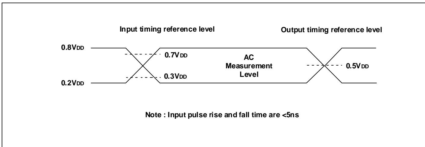
Figure 38: AC Input/Output Reference Waveforms
