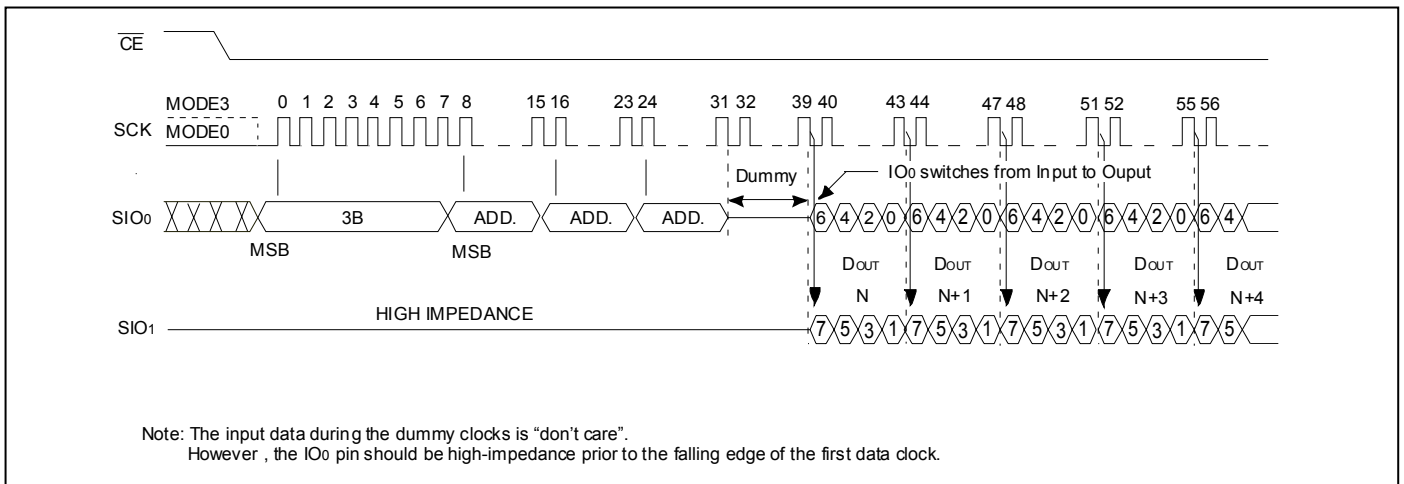
Figure 28: Fast Read Dual Output Sequence
