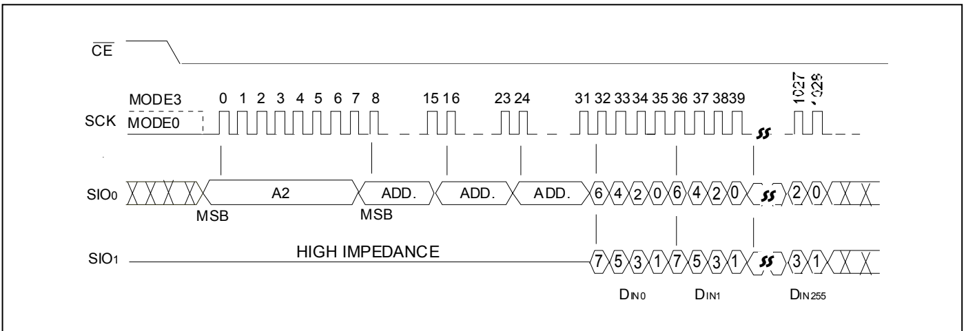
Figure 31: Dual Input Fast Program Sequence
