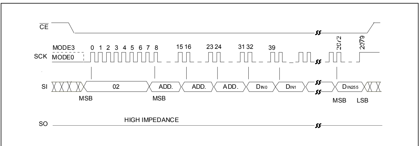
Figure 12-1: Page Program (PP) Sequence (SPI Mode)
