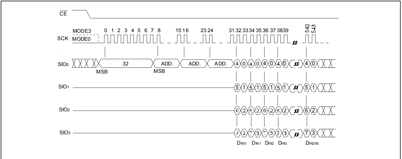
Figure 30: Quad Page Program (single address) Sequence
