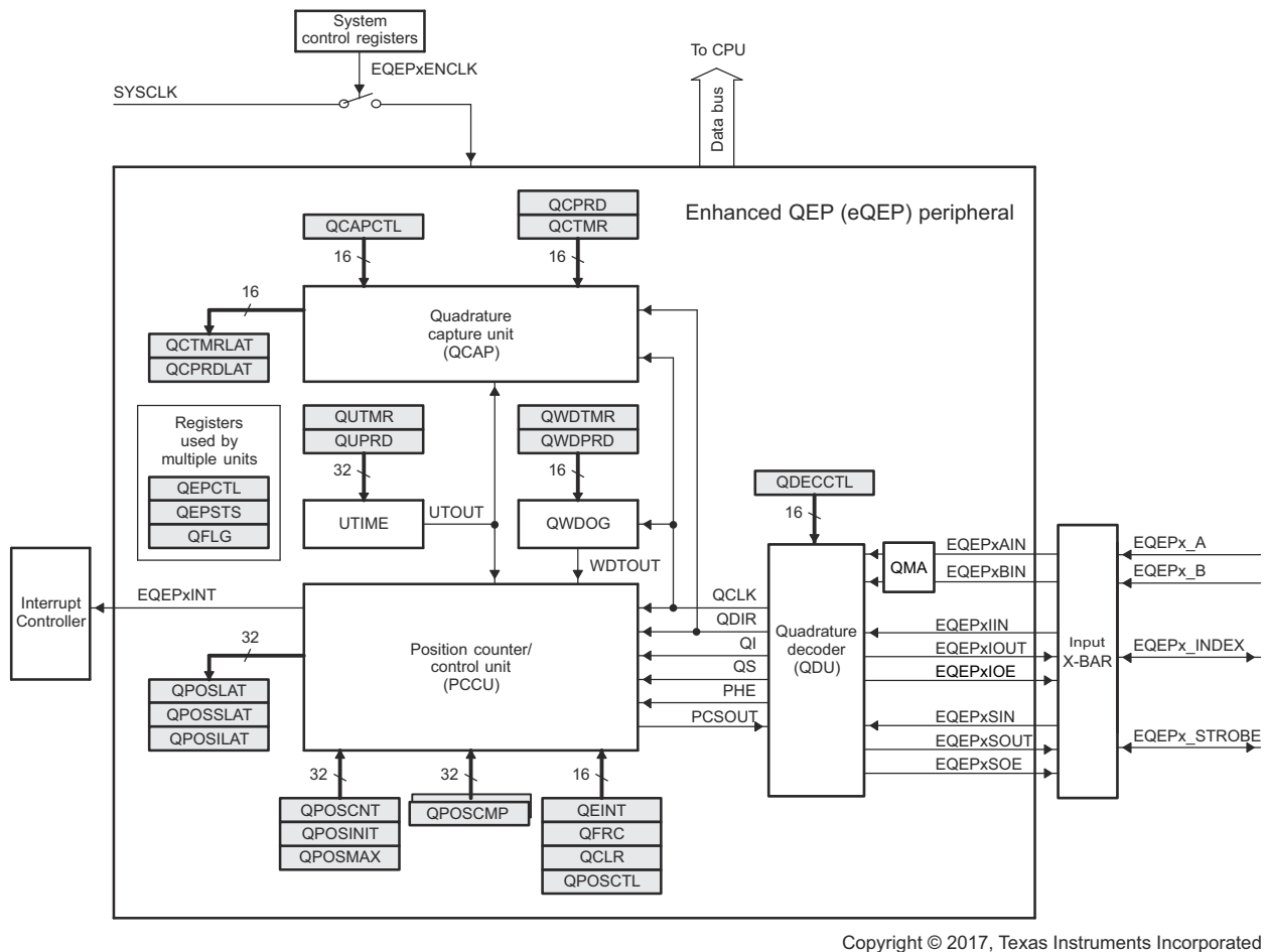
Figure 6-51. eQEP Block Diagram
