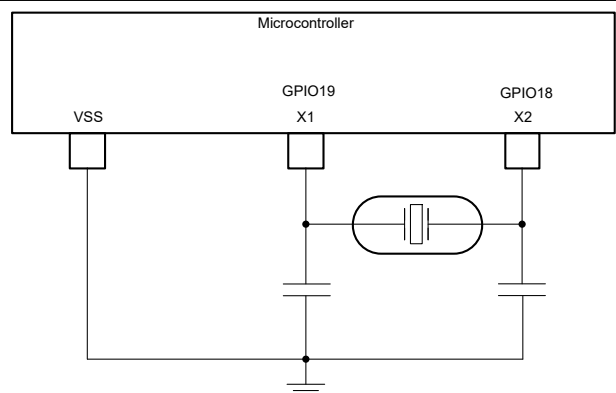
Figure 6-11. External Crystal
