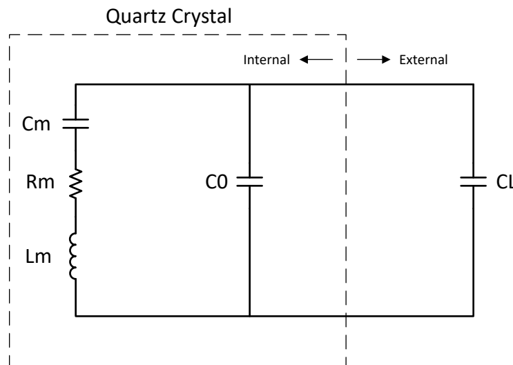
Figure 6-14. Crystal Electrical Representation
