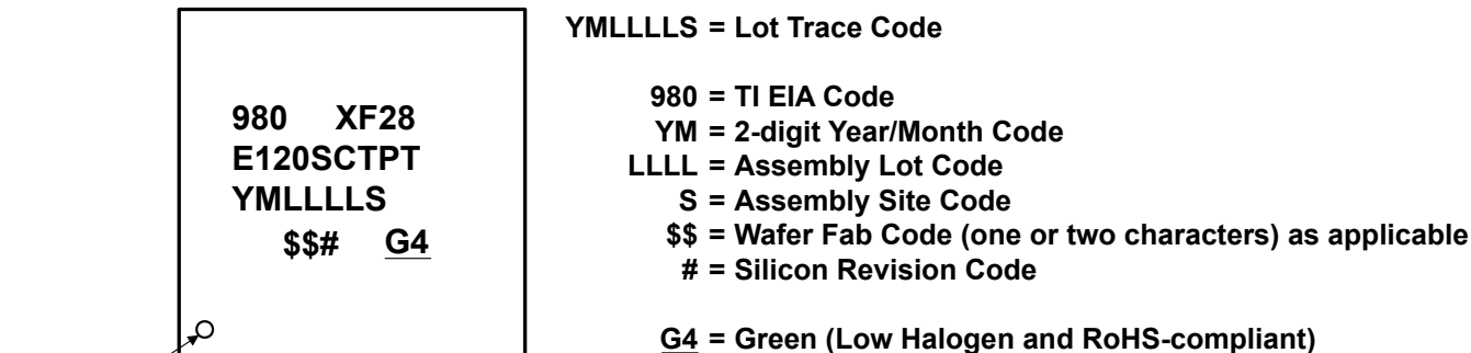
Figure 9-2. Package Symbolization for PT Package
