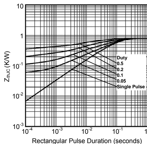
Fig6. Transient Thermal Impedance
