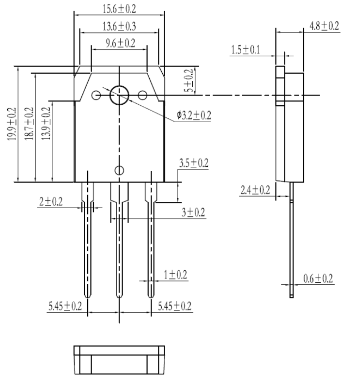
Dimensions in Millimeters Fig8. Package Outline
