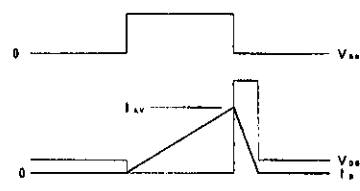
図2 動作波形 Operating waveforms
